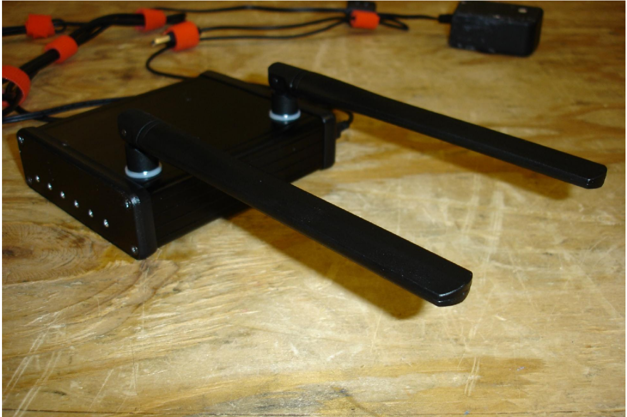
External view of the Hub's enclosure. Shows end plate with holes for LEDs and antenna mounting. Power supply in background.
