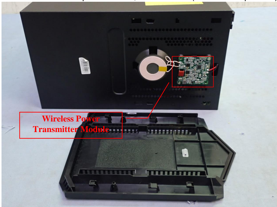
Personal Computer D19W6, Internal View (Removed Top Cover)
