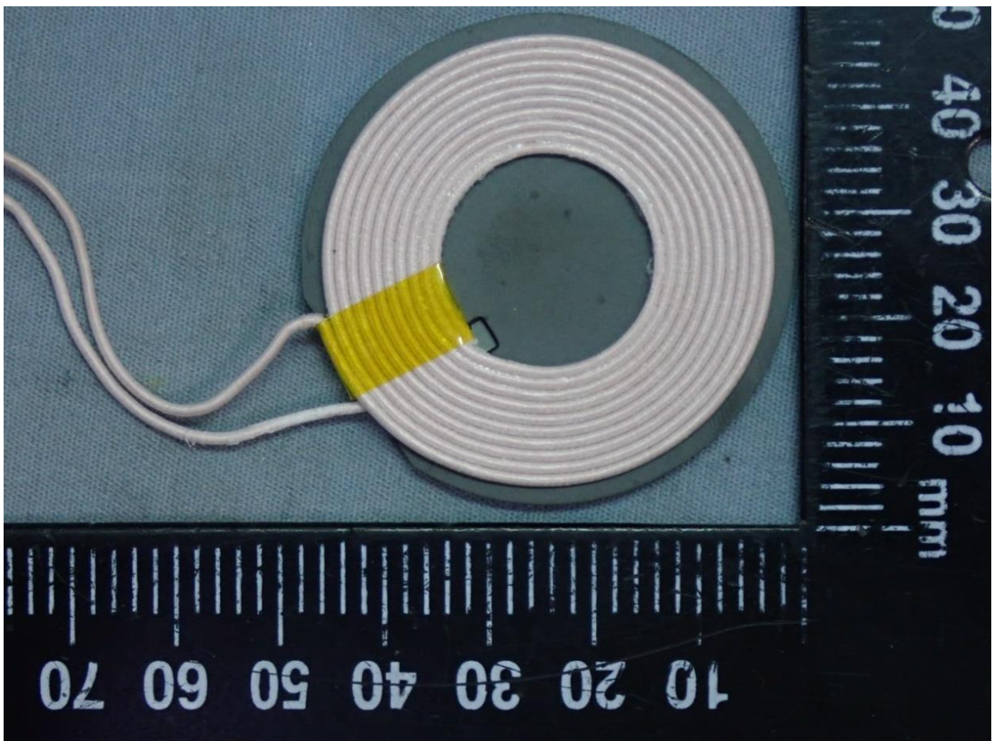
Figure 4 General Appearance (Antenna View)
