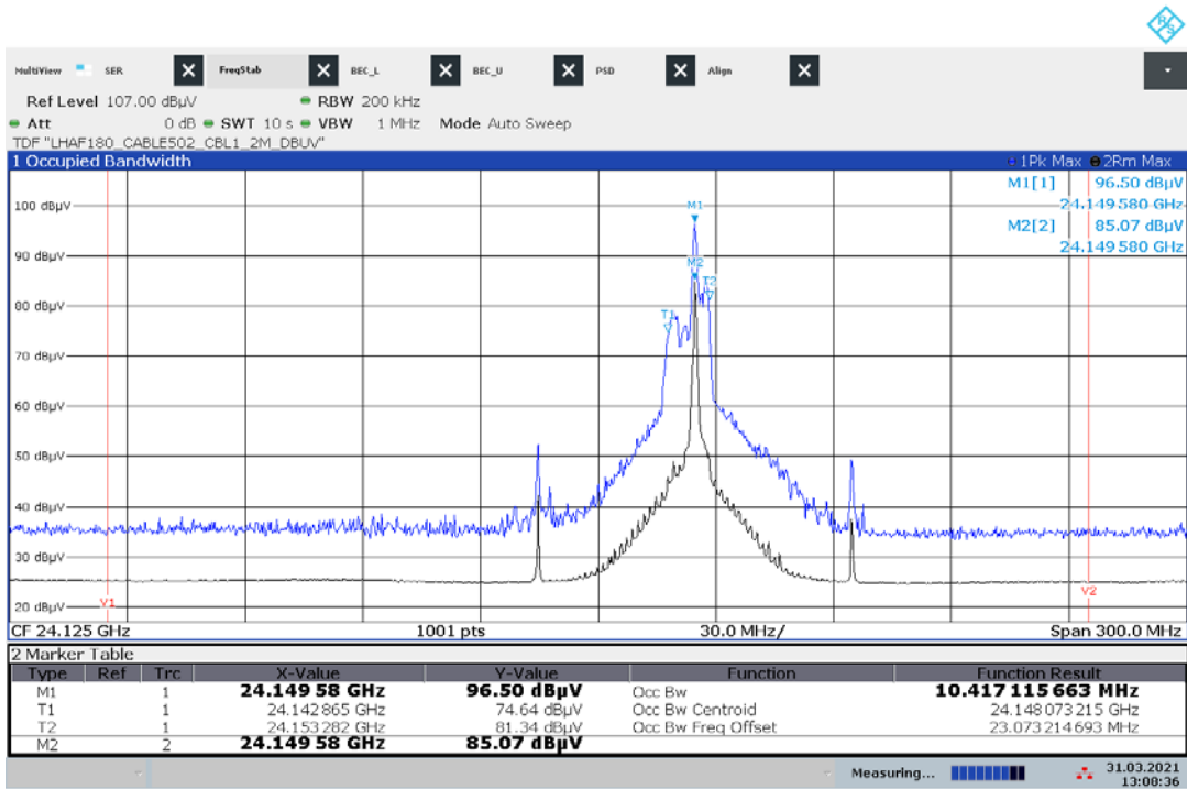
Plot 46: +20 °C, middle frequency mode, V_{nom}
