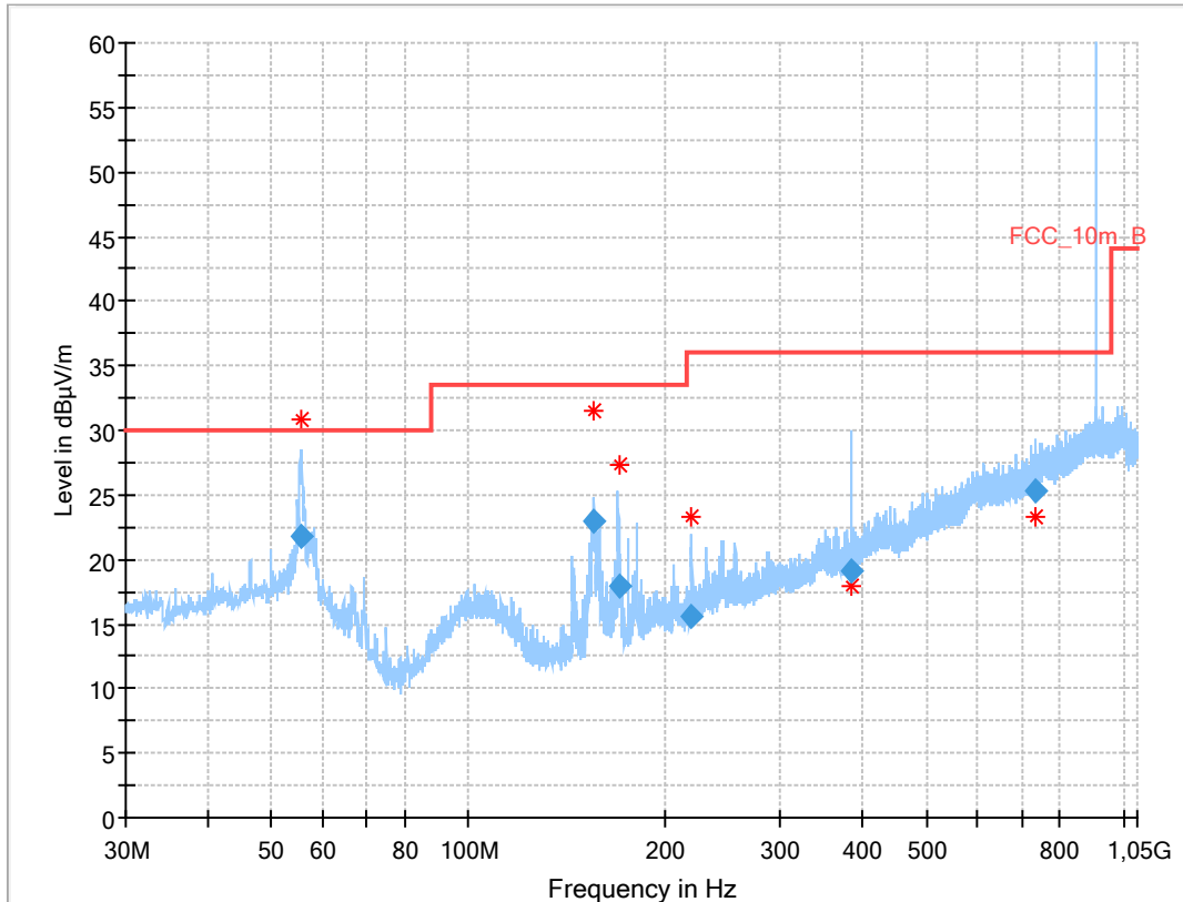
Plot No. 12: 30 MHz to 1 GHz, horizontal/vertical polarization, high channel
