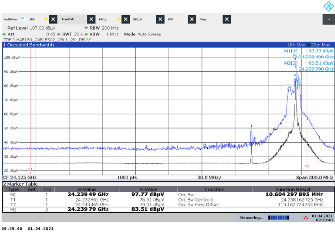
Plot 56: +35 °C, high frequency mode, V_{nom}
