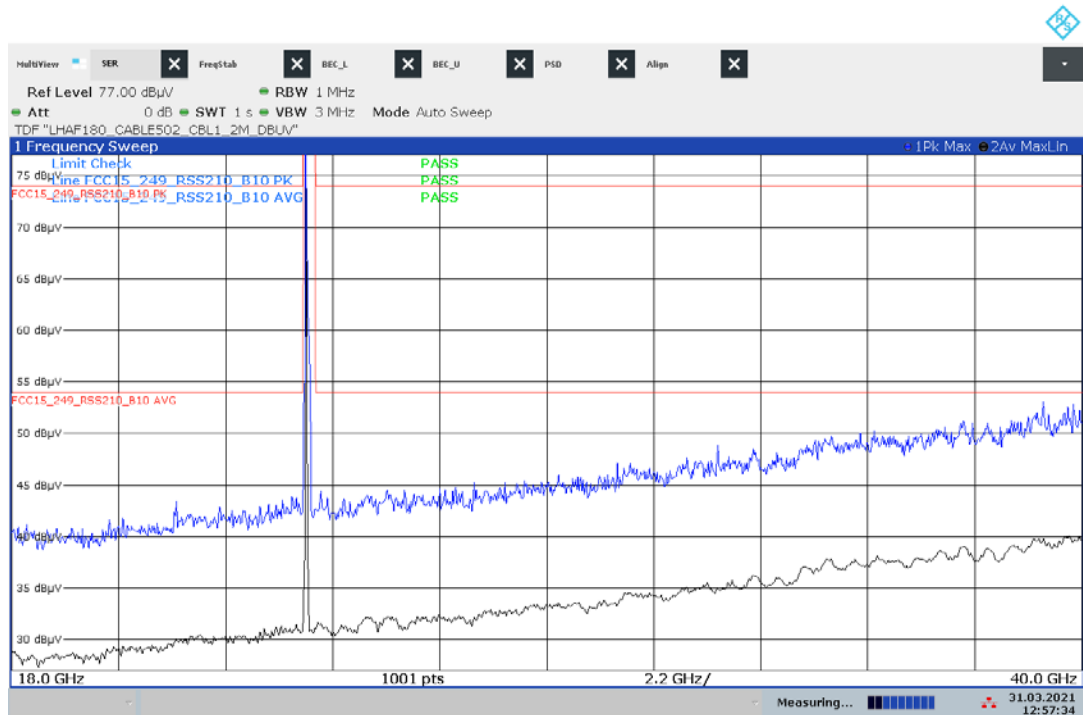
Plot No. 16: 18 GHz to 40 GHz, horizontal/vertical polarization, low channel
