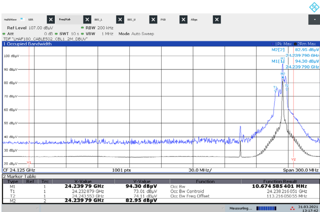
Plot 47: +20 °C, high frequency mode, V_{nom}
