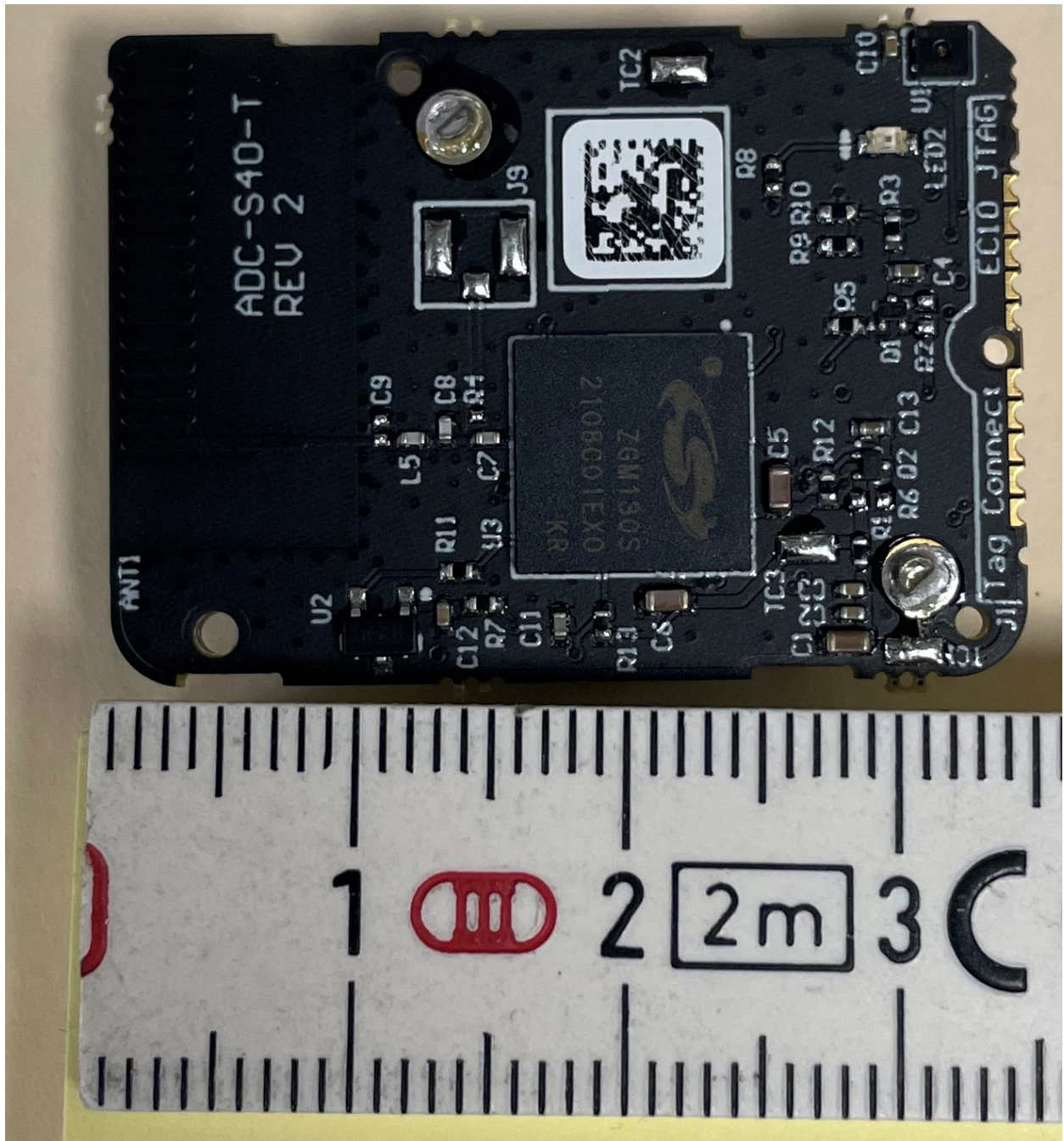
Internal Photos ADC-S40-T
