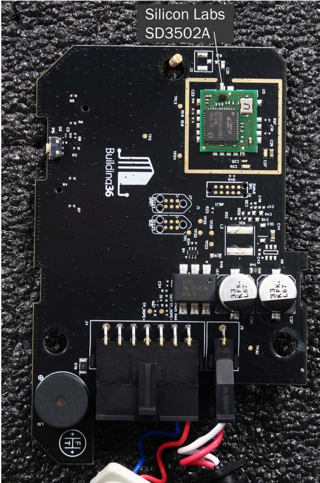
PCB Front
