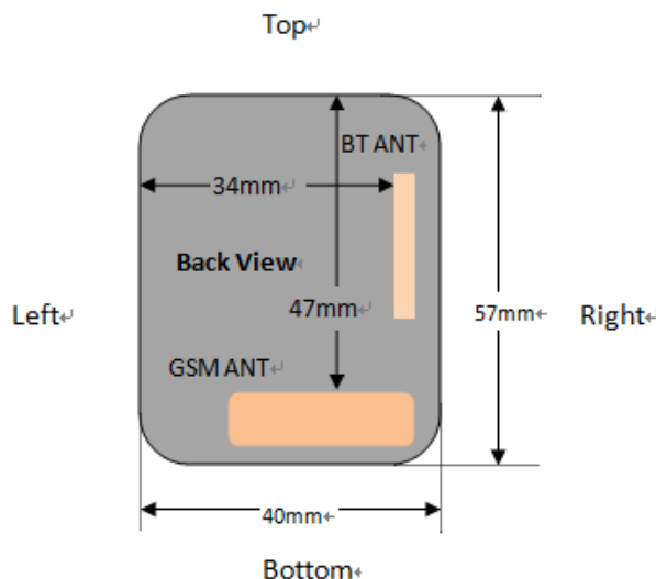
Fig.14.1 EUT Antenna Locations
