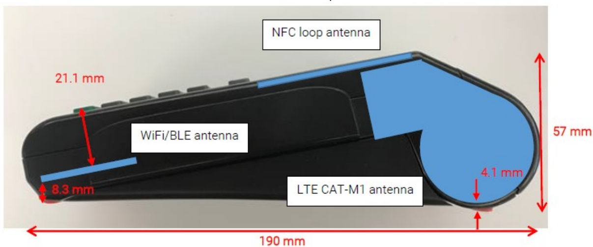
Photo 14: Antenna positions
