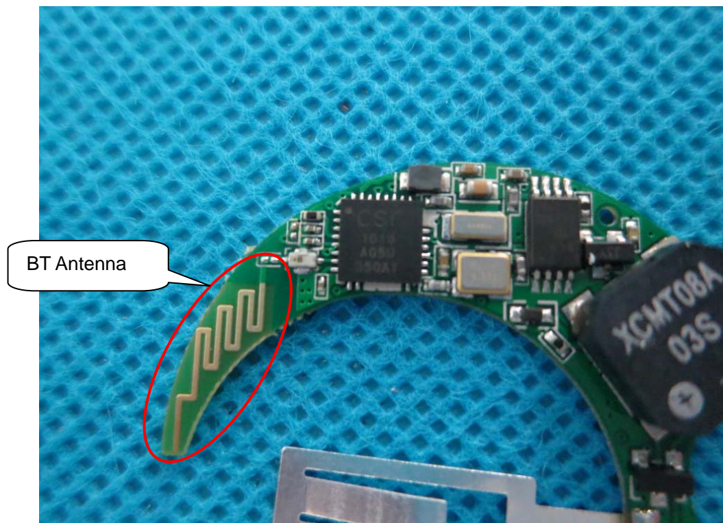
INTERNAL VIEW OF EUT (lithium cell)-4
