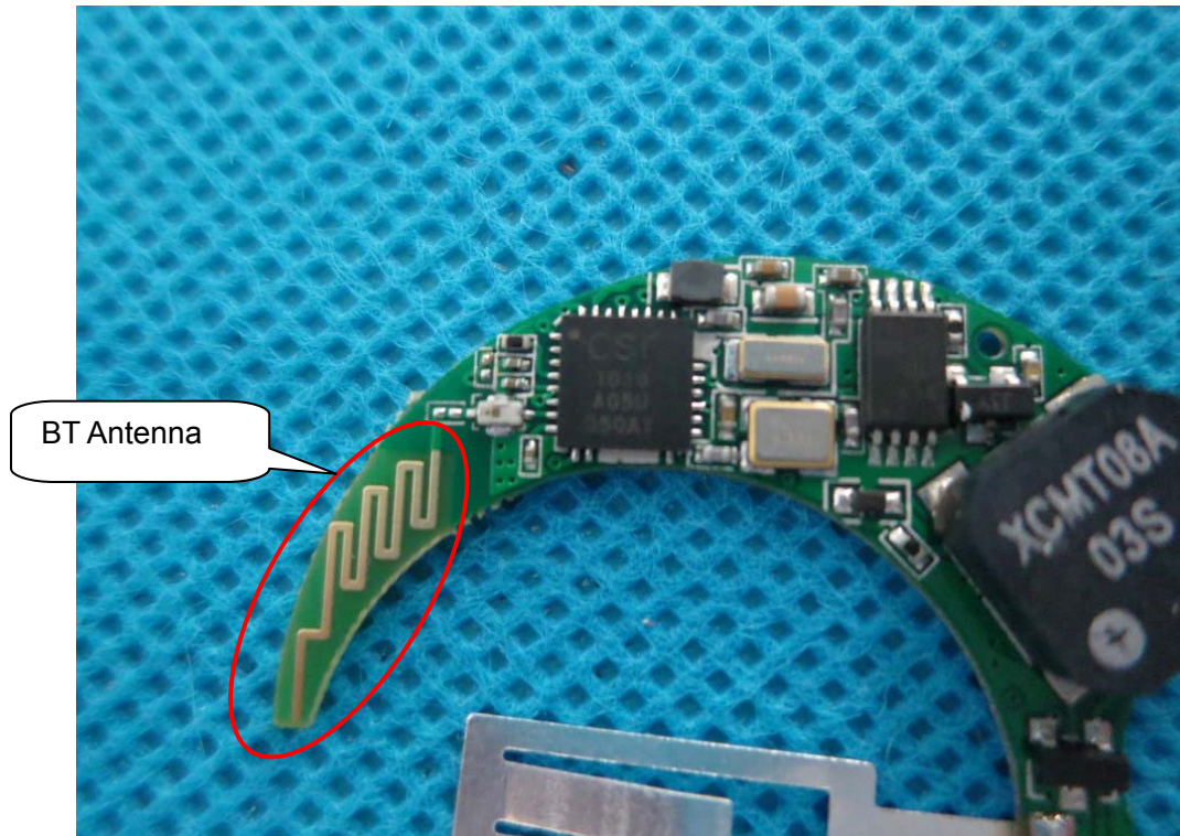
INTERNAL VIEW OF EUT (lithium cell)-4
