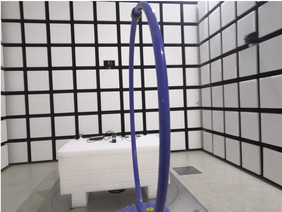
Radiated Emission 9kHz~30MHz Coplanar View
