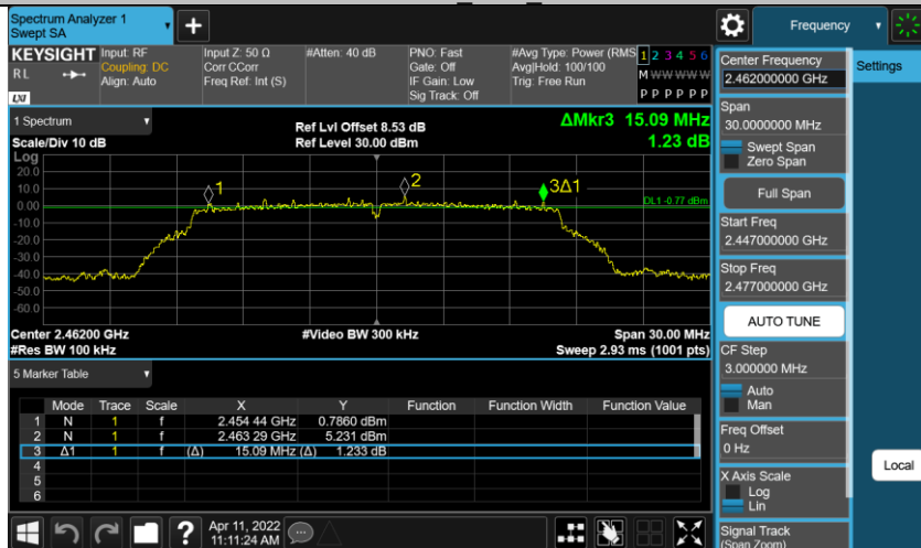
11G-SISO Ant2_2462
