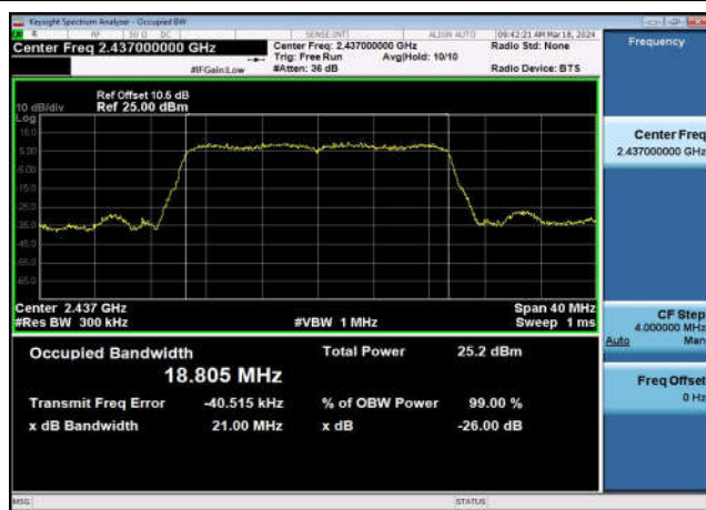
99% Bandwidth-802.11ax(20MHz),2437MHz ,Ant0
