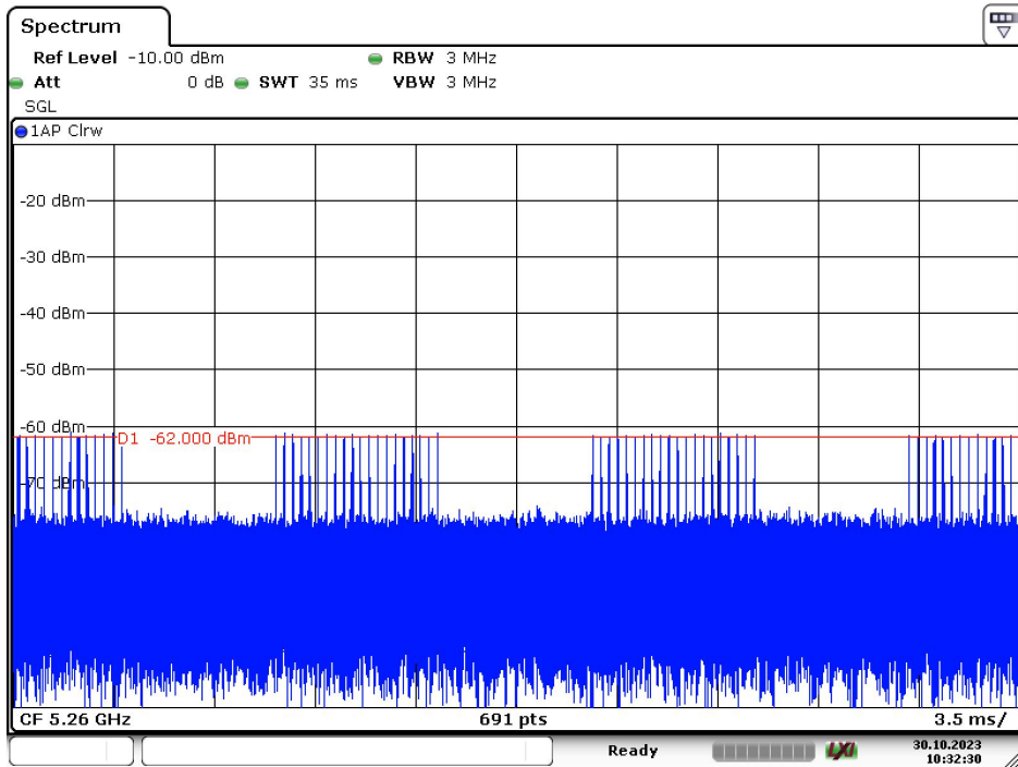
Radar Type 4 – 5260MHz
