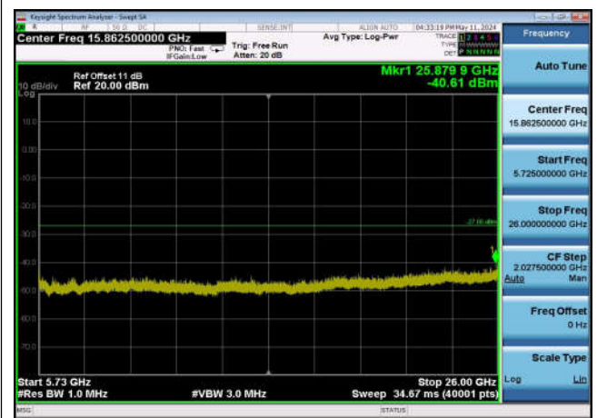
U-NII-2c ,Plot 1,Band Edge-802.11a(20 MHz),5600MHz,Ant0
