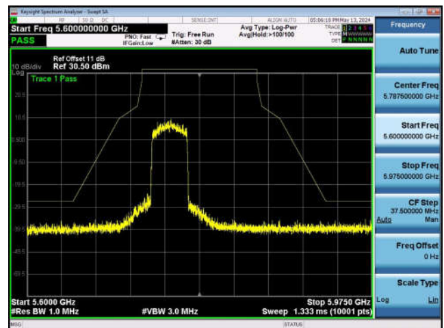
U-NII-3 ,Plot 1,Band Edge-802.11ax(80 MHz),5775MHz,Ant0
