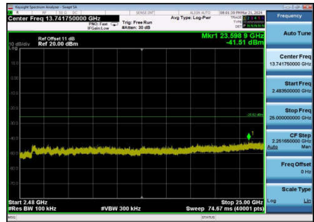
,Plot 4,2483.5MHz~25000MHz-802.11g ,2462MHz,Ant1
