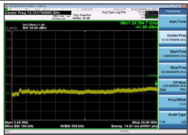
,Plot 4,2483.5MHz~25000MHz-802.11n(40 MHz),2437MHz,Ant1
