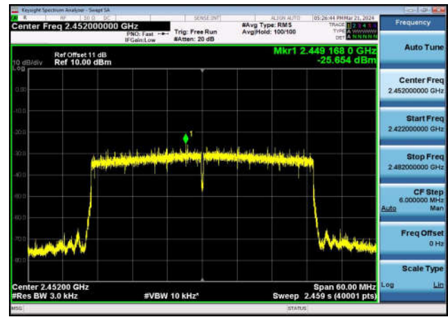
Power spectral density-802.11ax(40MHz),2452MHz,Ant1
