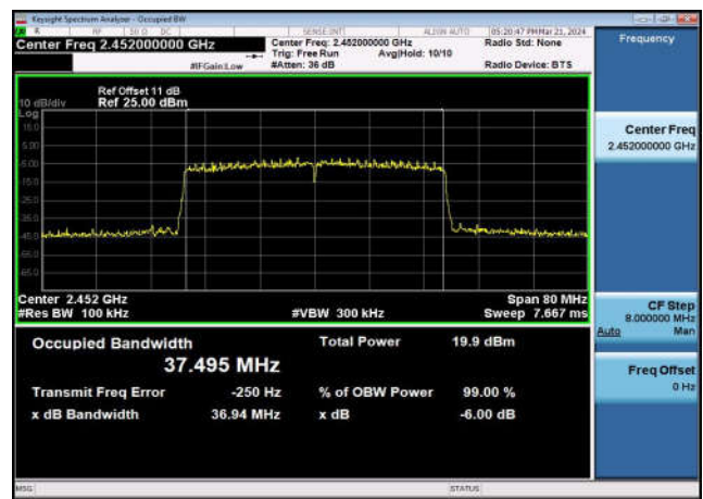
6dB Bandwidth-802.11ax(40MHz),2452MHz ,Ant1
