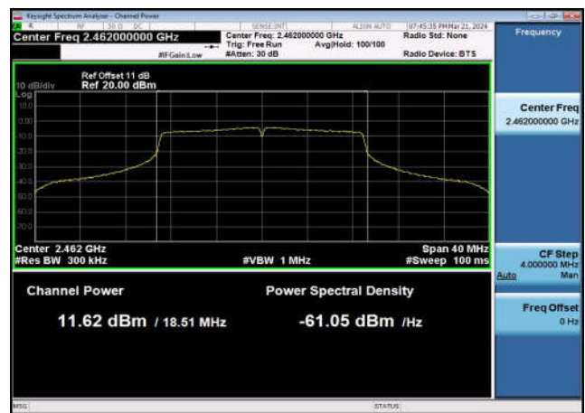
Output Power-802.11n(40MHz),2422MHz ,Ant1
