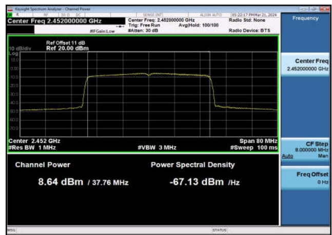
Output Power-802.11ax(40MHz),2452MHz ,Ant1
