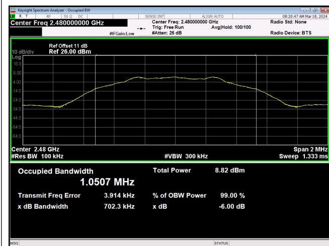
1Mbps_Channel 39
