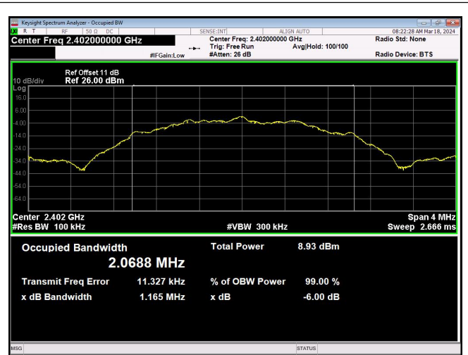
2Mbps_Channel 0
