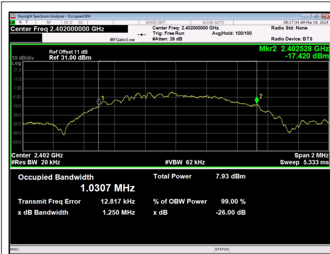
1Mbps_Channel 0
