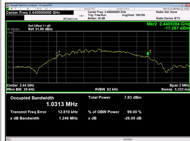
1Mbps_Channel 19
