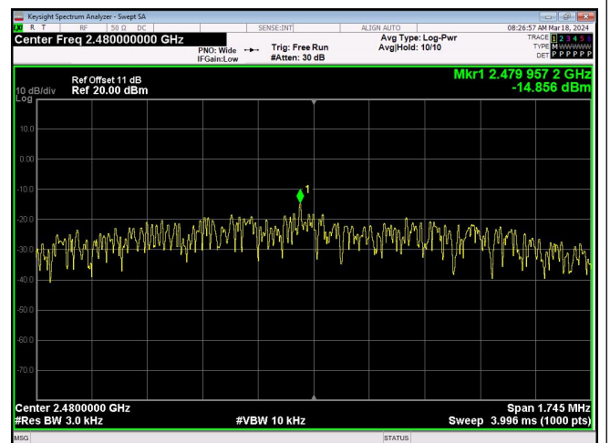
2Mbps_Channel 39
