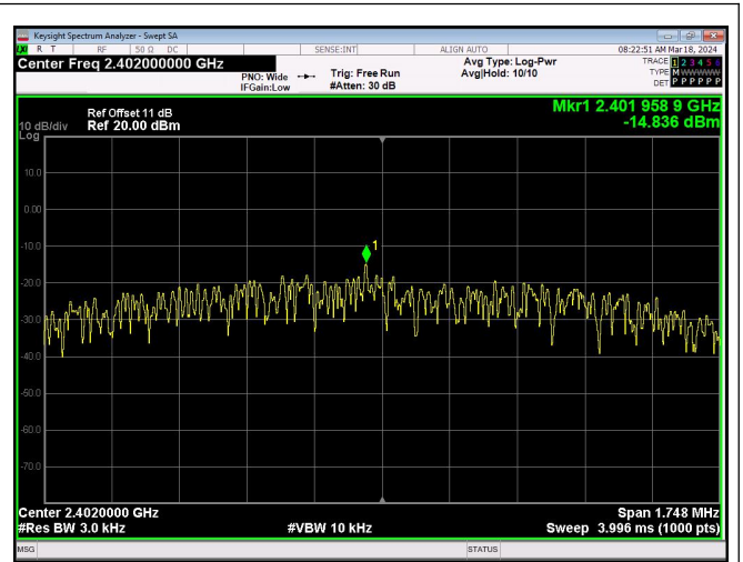
2Mbps_Channel 0
