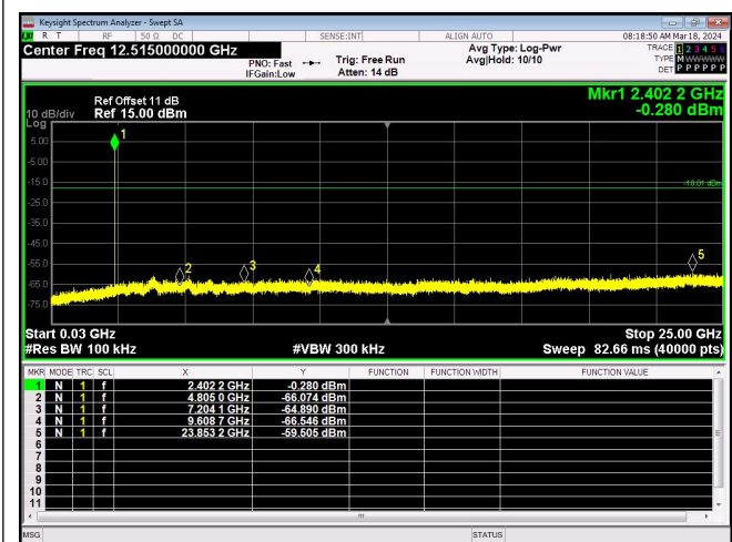
Spurious Emission 1Mbps_Channel 0
