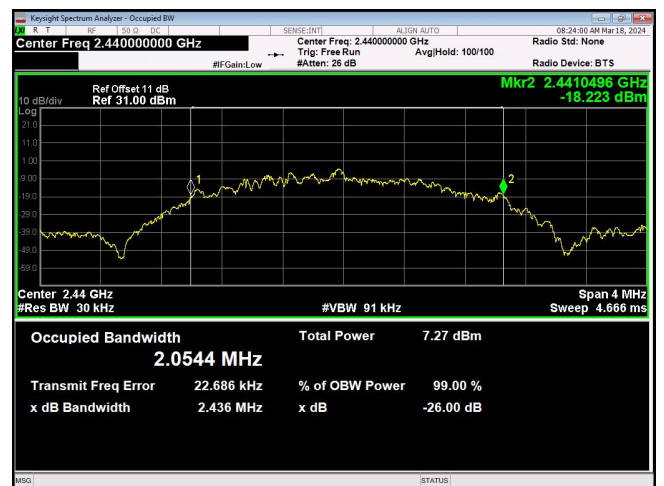
2Mbps_Channel 19
