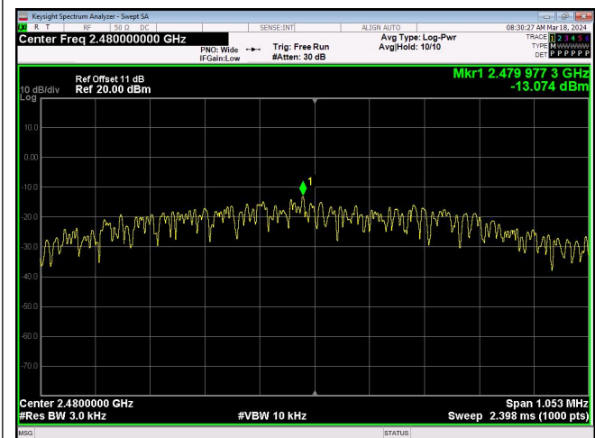
1Mbps_Channel 39
