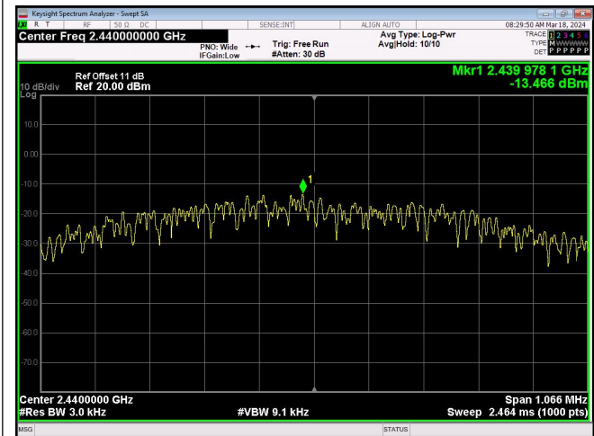
1Mbps_Channel 19
