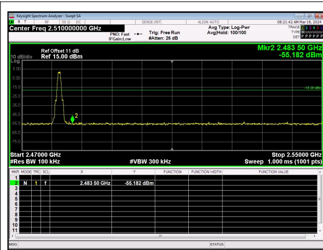
Out Of Band Emission 1Mbps_Channel 39
