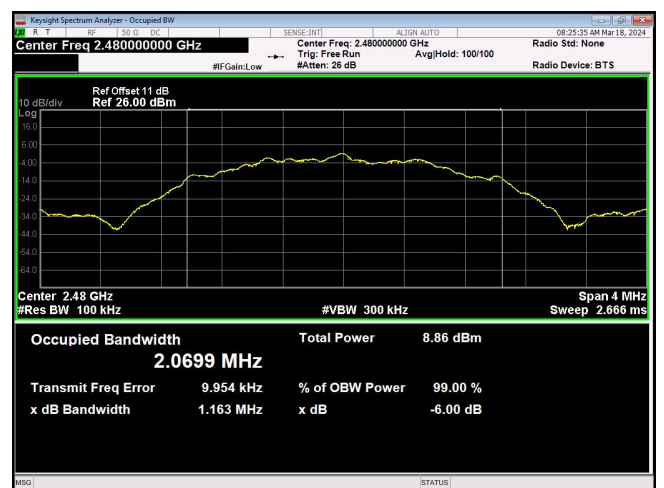
2Mbps_Channel 39
