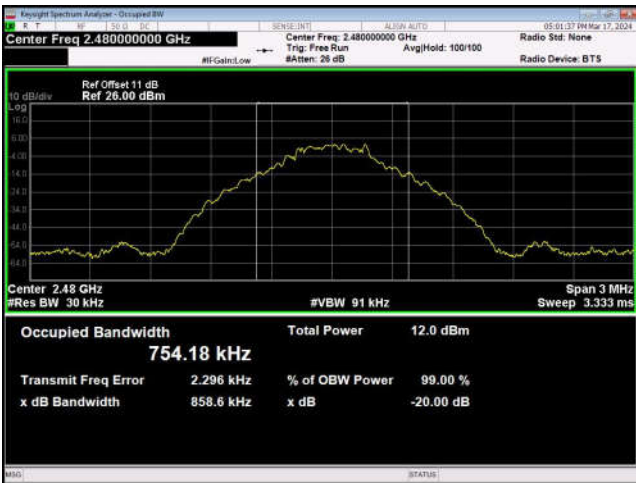
GFSK_DH5_Channel 78
