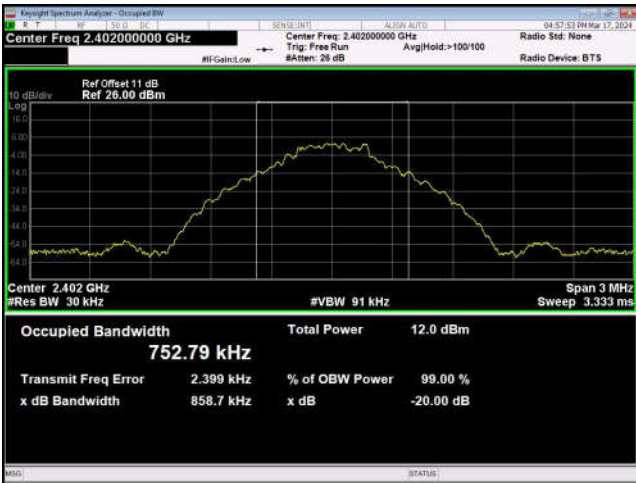
GFSK_DH5_Channel 0
