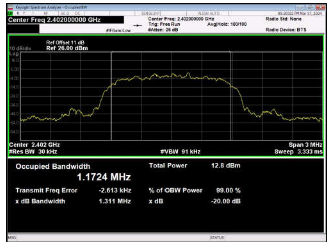
\pi/4 DQPSK_2-DH5_Channel 0
