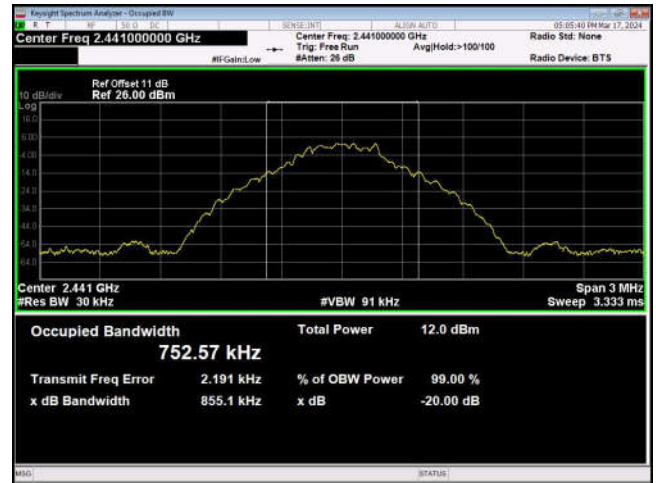
GFSK_DH5_Channel 39
