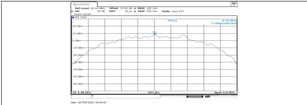
BLE_2M_Ant1_2480_0~Reference
