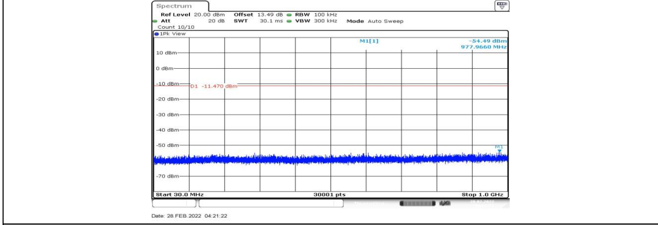
BLE_1M_Ant1_2480_30~100
