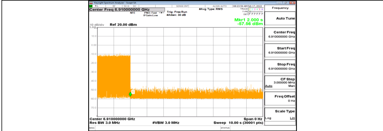
11AX80MIMO_Ant1_6945_High_6910_10
