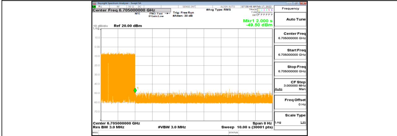
11AX80MIMO_Ant1_6705_Center_6705_2
