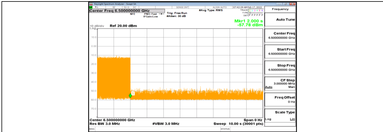
11AX80MIMO_Ant1_6465_Low_6500_9
