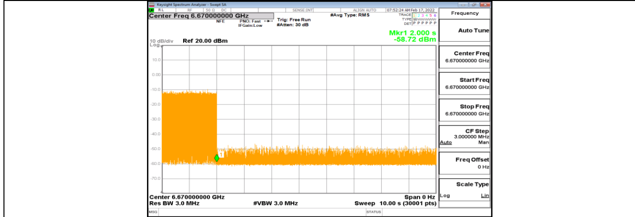
11AX80MIMO_Ant1_6705_High_6670_4
