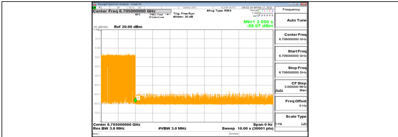
11AX80MIMO_Ant1_6705_Center_6705_7
