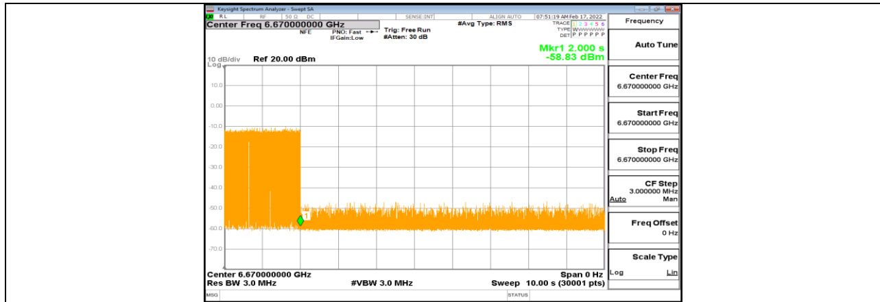
11AX80MIMO_Ant1_6705_High_6670_2
