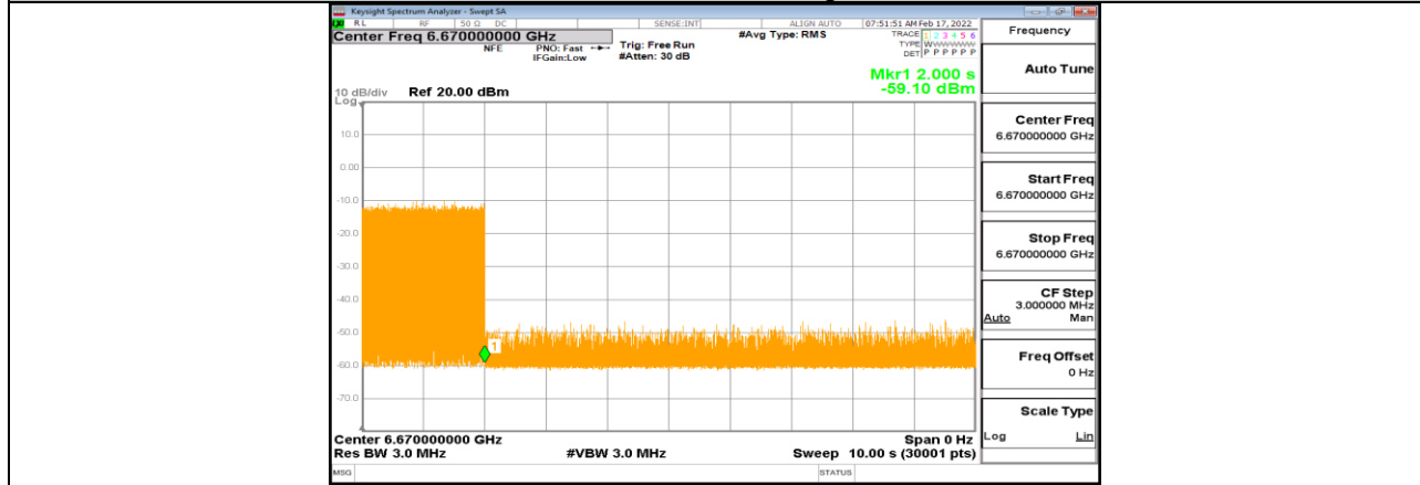
11AX80MIMO_Ant1_6705_High_6670_3
