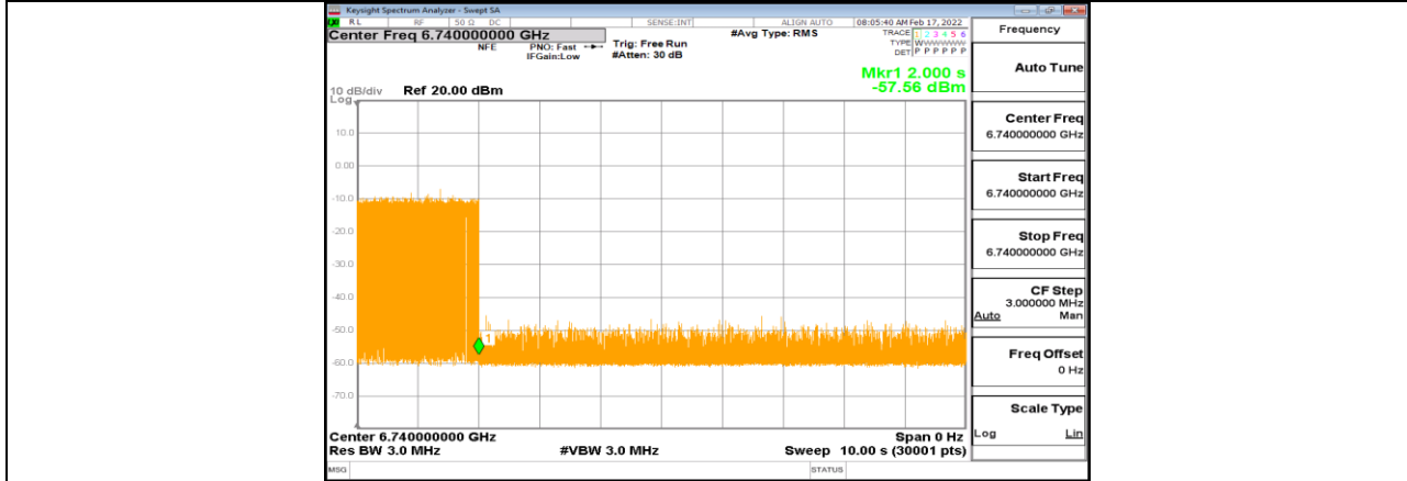
11AX80MIMO_Ant1_6705_Low_6740_2
