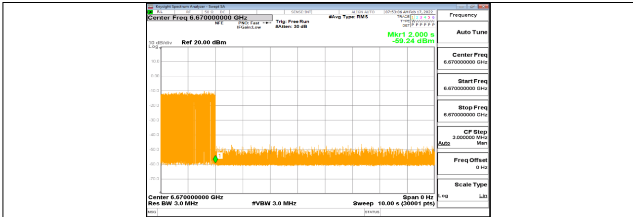
11AX80MIMO_Ant1_6705_High_6670_5
