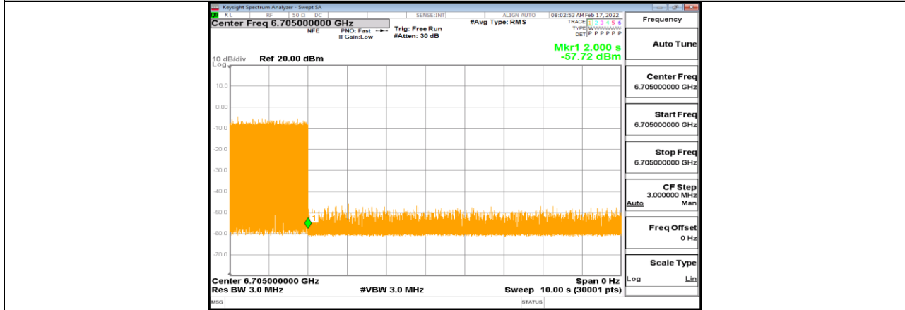
11AX80MIMO_Ant1_6705_Center_6705_8
