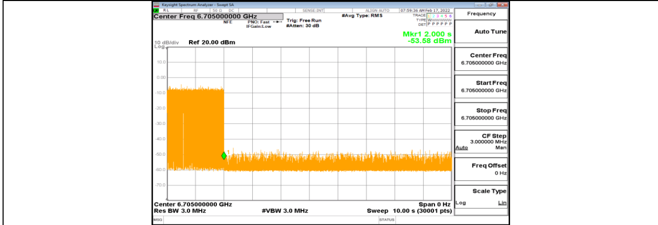
11AX80MIMO_Ant1_6705_Center_6705_3
