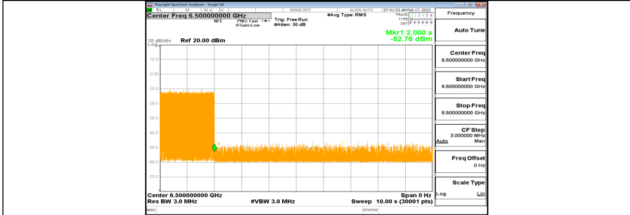
11AX80MIMO_Ant1_6465_Low_6500_8
