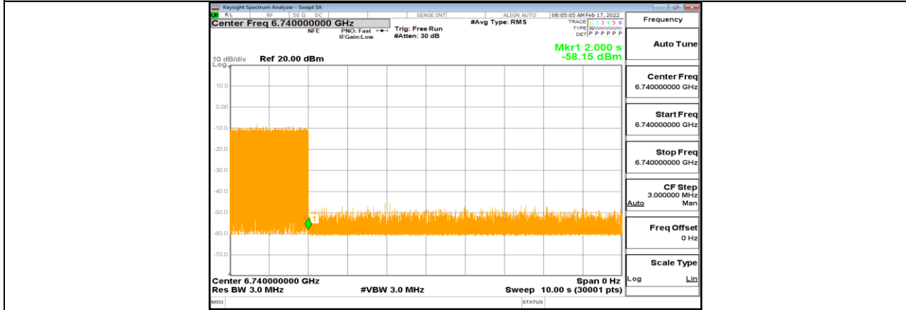
11AX80MIMO_Ant1_6705_Low_6740_1
