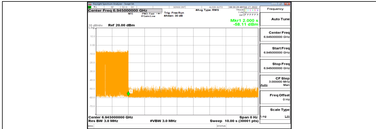
11AX80MIMO_Ant1_6945_Center_6945_7
