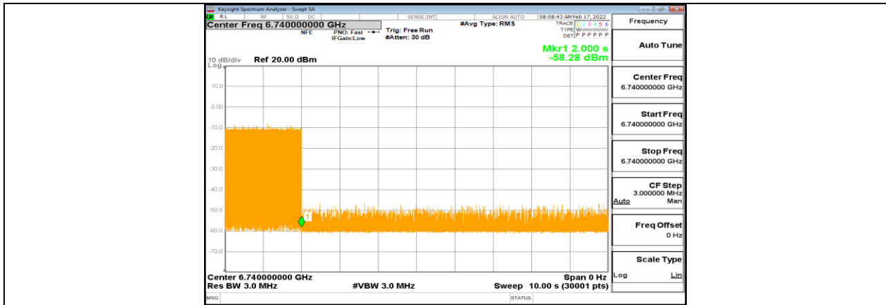
11AX80MIMO_Ant1_6705_Low_6740_6
