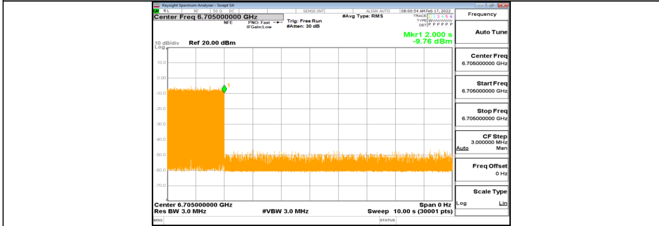
11AX80MIMO_Ant1_6705_Center_6705_5
