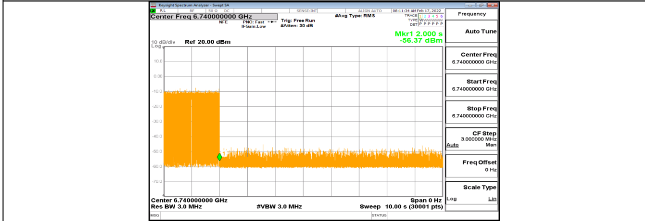
11AX80MIMO_Ant1_6705_Low_6740_10
