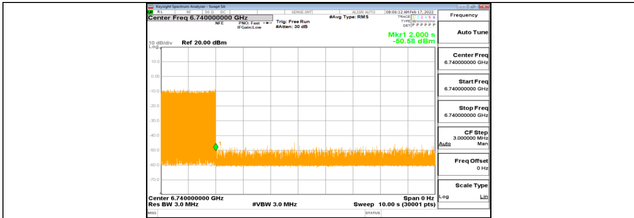
11AX80MIMO_Ant1_6705_Low_6740_3
