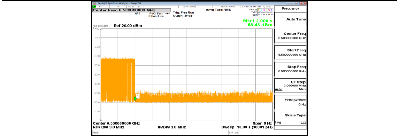
11AX80MIMO_Ant1_6465_Low_6500_7
