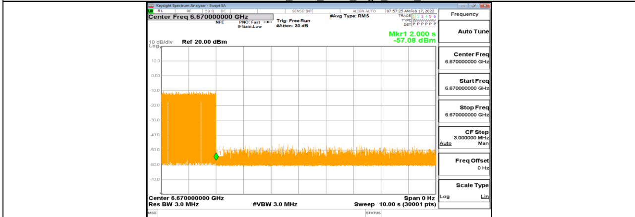
11AX80MIMO_Ant1_6705_High_6670_10
