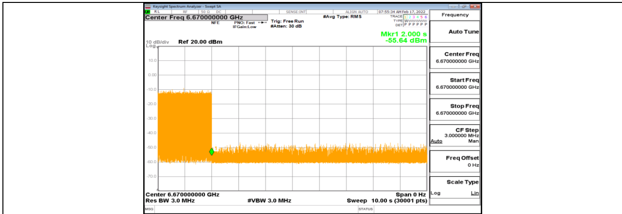
11AX80MIMO_Ant1_6705_High_6670_8
