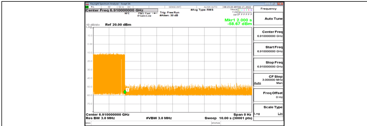
11AX80MIMO_Ant1_6945_High_6910_2
