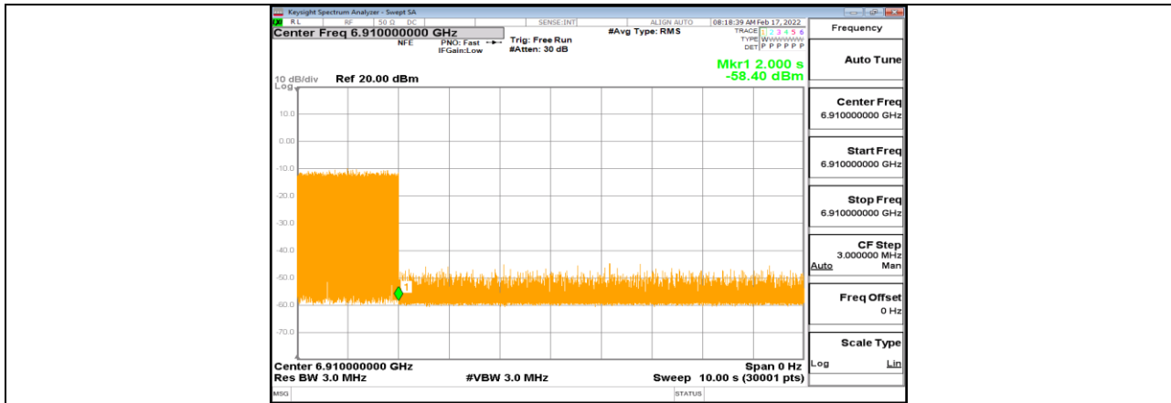
11AX80MIMO_Ant1_6945_High_6910_5
