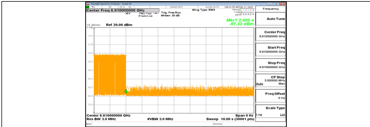
11AX80MIMO_Ant1_6945_High_6910_8
