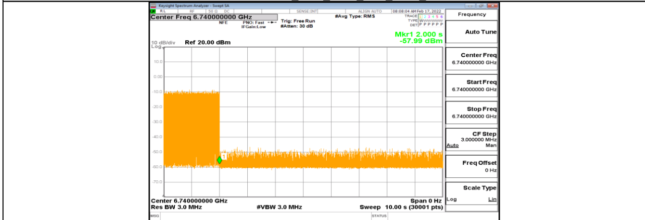
11AX80MIMO_Ant1_6705_Low_6740_5
