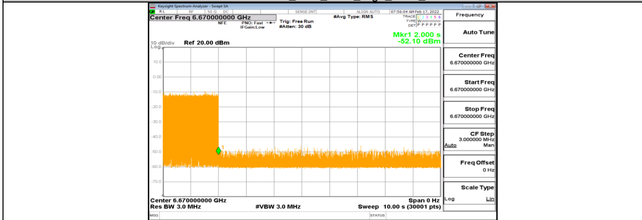
11AX80MIMO_Ant1_6705_High_6670_9
