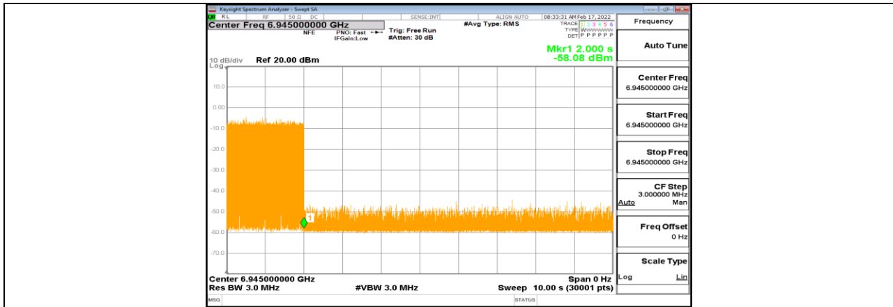
11AX80MIMO_Ant1_6945_Center_6945_10
