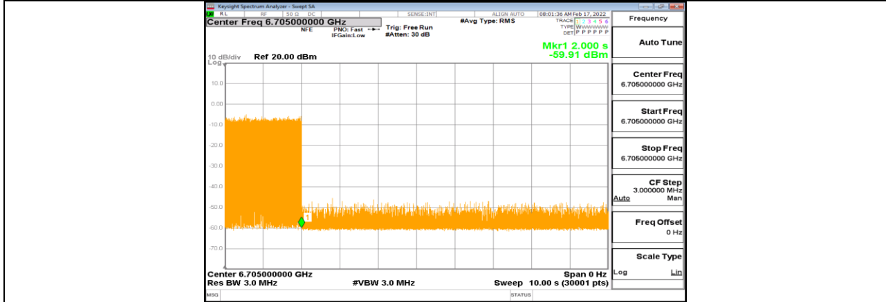
11AX80MIMO_Ant1_6705_Center_6705_6
