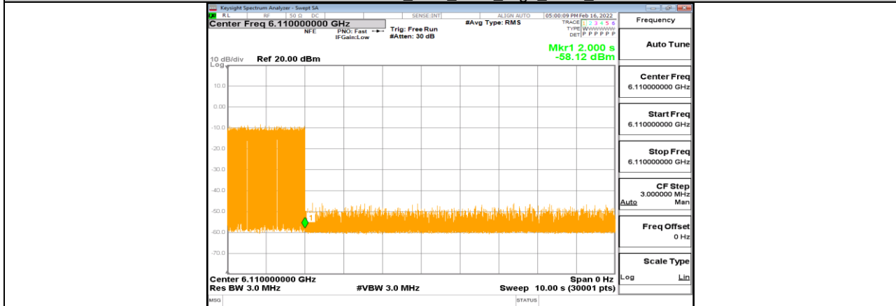
11AX80MIMO_Ant1_6145_High_6110_7
