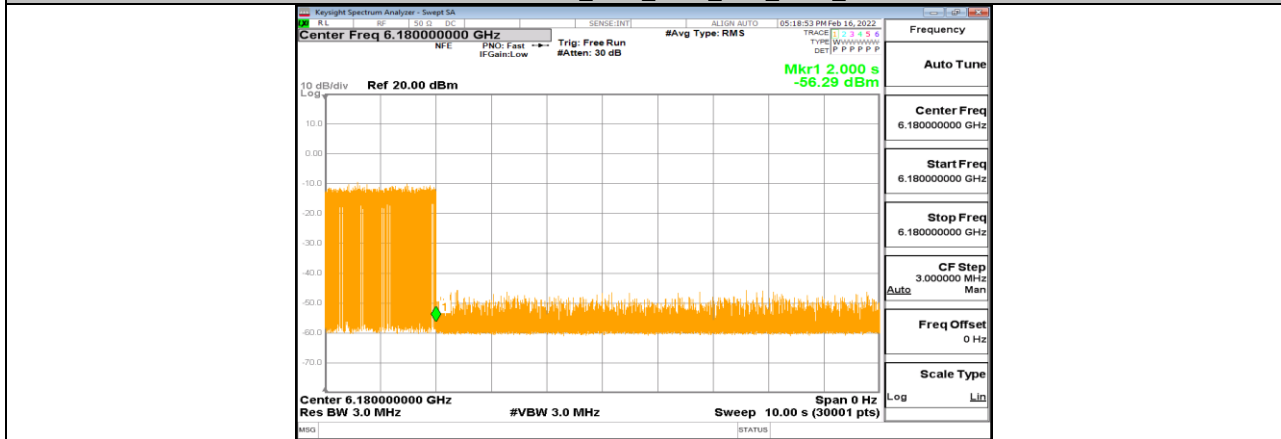
11AX80MIMO_Ant1_6145_Low_6180_10
