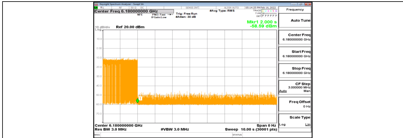
11AX80MIMO_Ant1_6145_Low_6180_3
