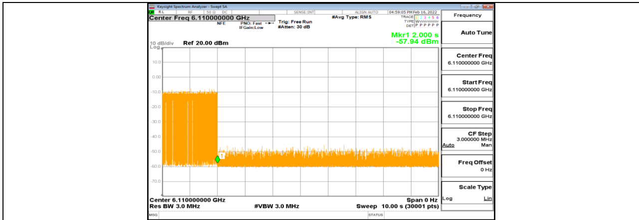
11AX80MIMO_Ant1_6145_High_6110_5
