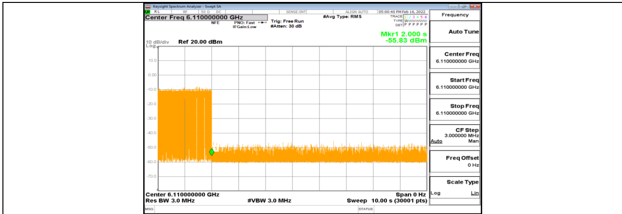
11AX80MIMO_Ant1_6145_High_6110_8
