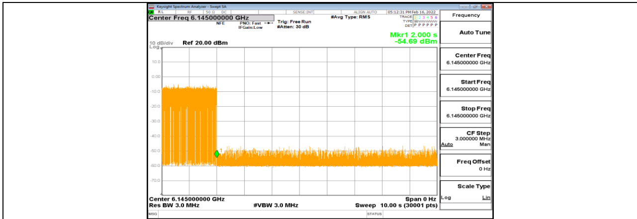
11AX80MIMO_Ant1_6145_Center_6145_10
