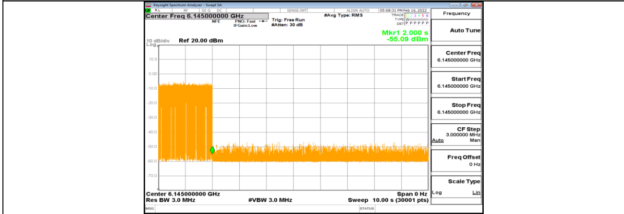
11AX80MIMO_Ant1_6145_Center_6145_5
