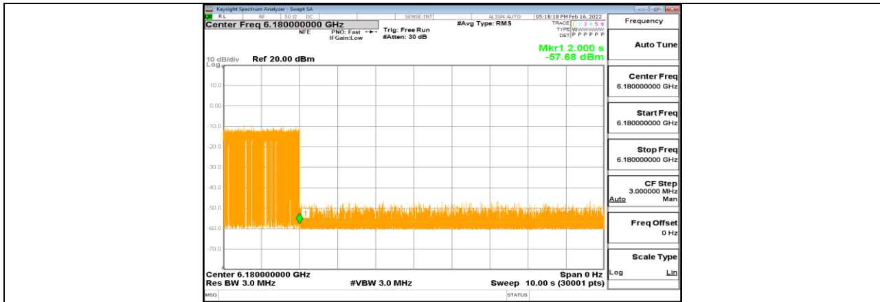
11AX80MIMO_Ant1_6145_Low_6180_9
