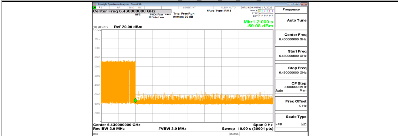
11AX80MIMO_Ant1_6465_High_6430_1
