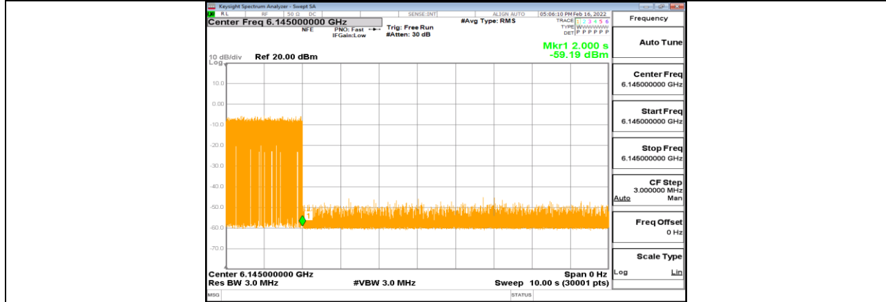
11AX80MIMO_Ant1_6145_Center_6145_3
