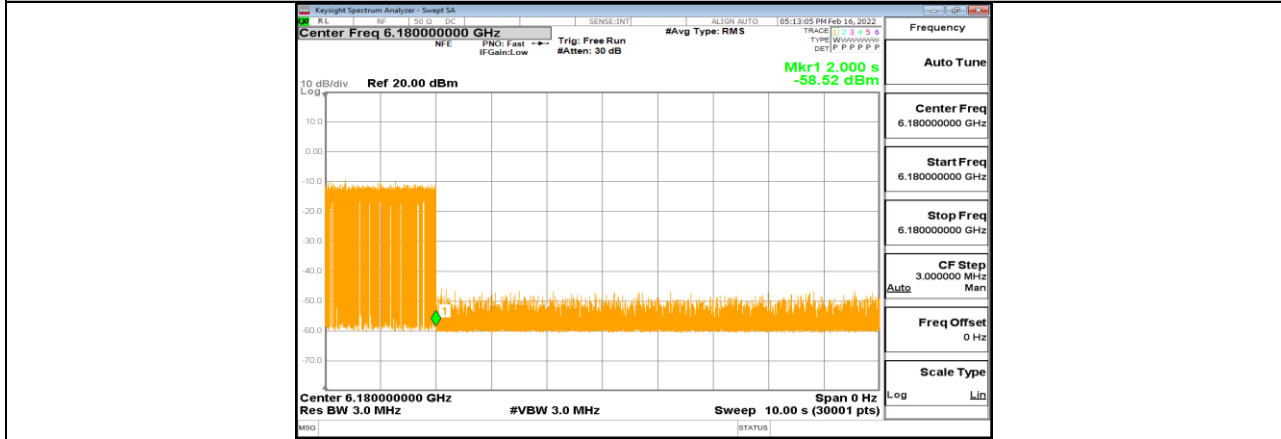
11AX80MIMO_Ant1_6145_Low_6180_1
