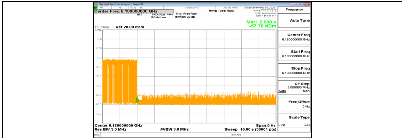
11AX80MIMO_Ant1_6145_Low_6180_6
