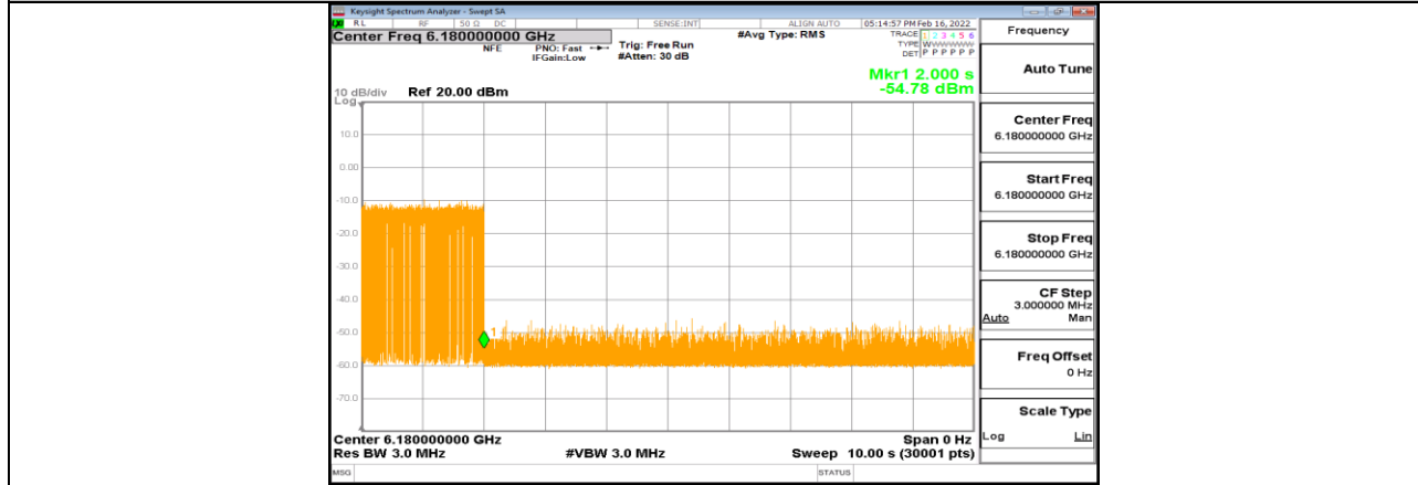
11AX80MIMO_Ant1_6145_Low_6180_4
