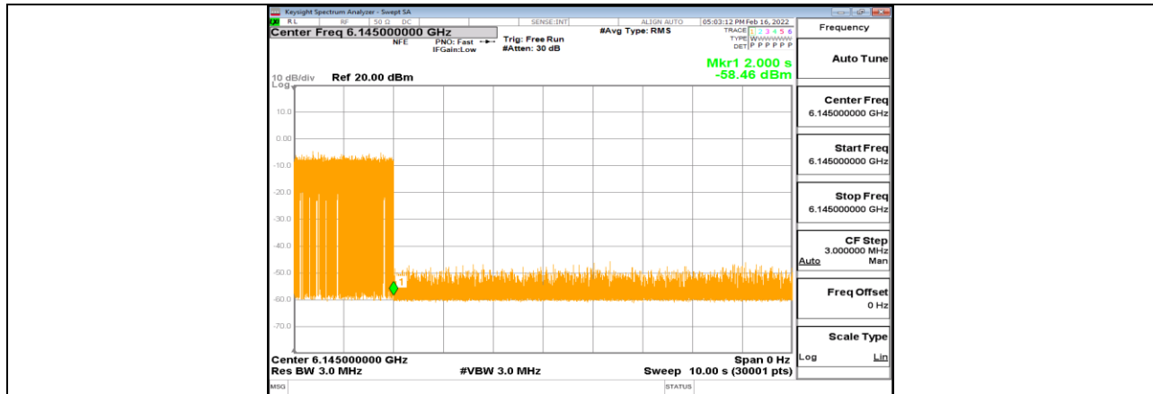
11AX80MIMO_Ant1_6145_Center_6145_1
