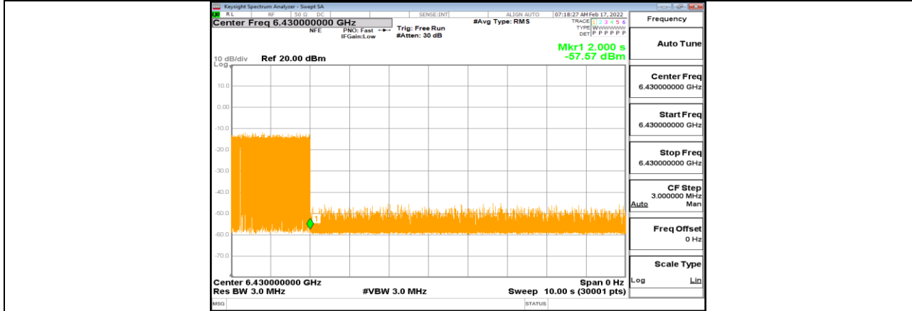
11AX80MIMO_Ant1_6465_High_6430_4
