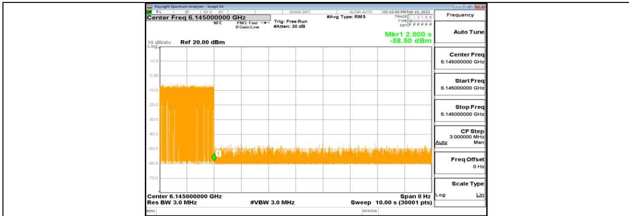
11AX80MIMO_Ant1_6145_Center_6145_7
