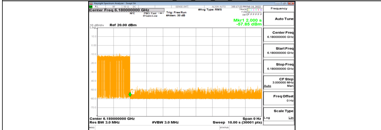
11AX80MIMO_Ant1_6145_Low_6180_8
