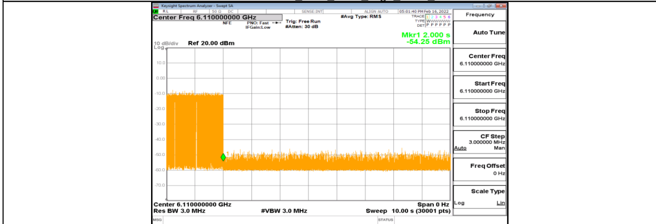
11AX80MIMO_Ant1_6145_High_6110_10
