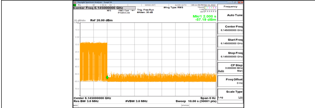
11AX80MIMO_Ant1_6145_Center_6145_9
