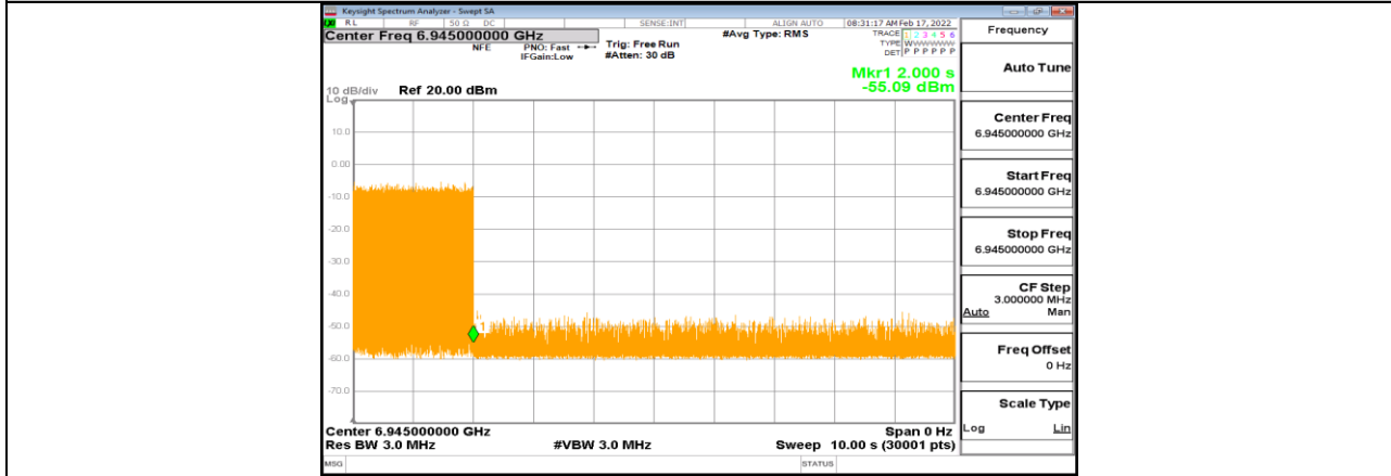
11AX80MIMO_Ant1_6945_Center_6945_8
