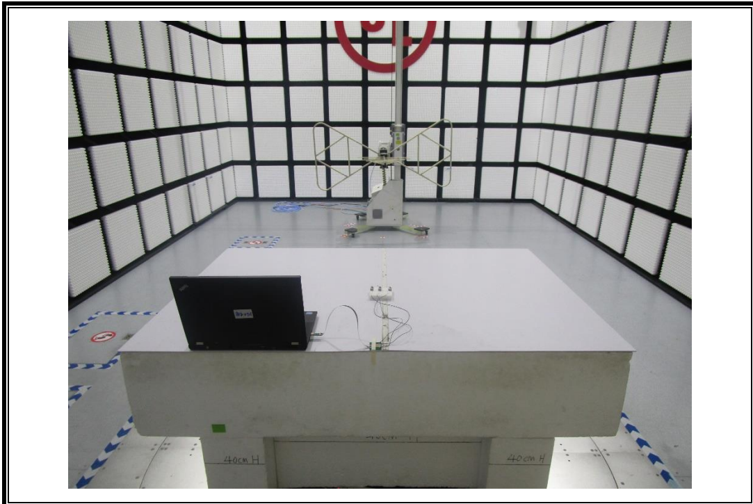
RADIATED RF MEASUREMENT SETUP (Below 1 GHz)
