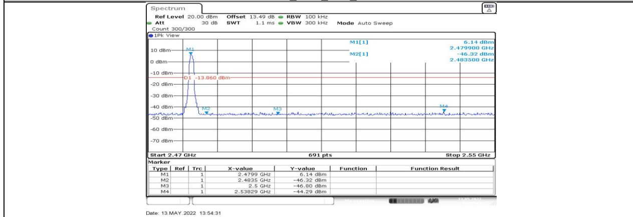
3DH5_Ant1_High_2480
