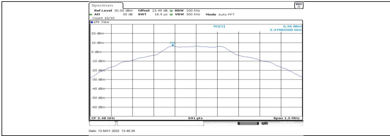
DH5_Ant1_2480_0~Reference
