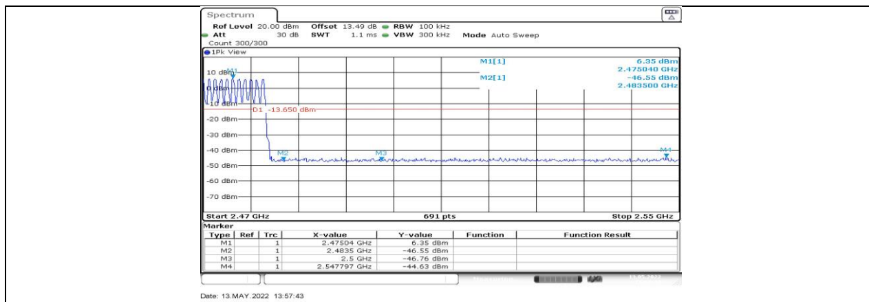
DH5_Ant1_High_Hop_2480
