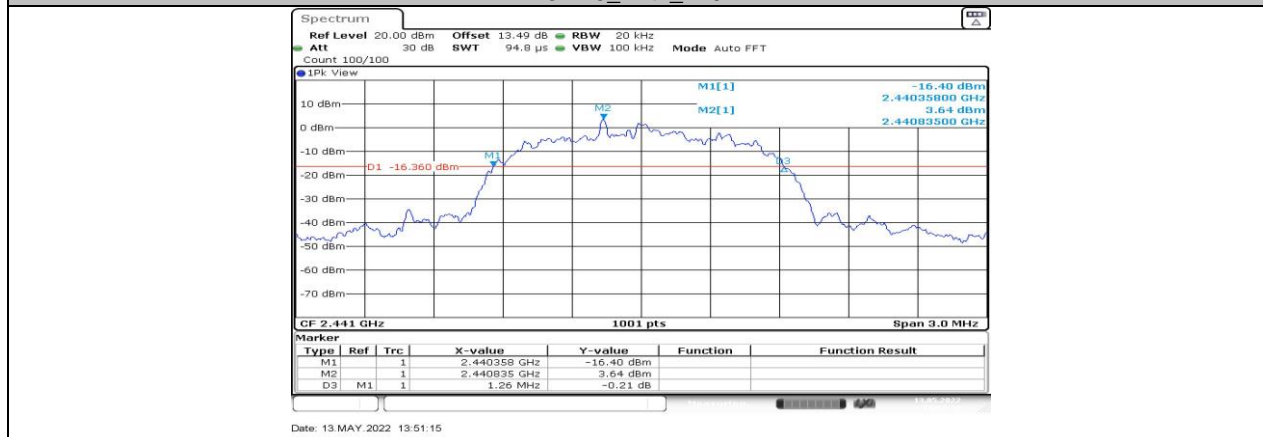
3DH5_Ant1_2441
