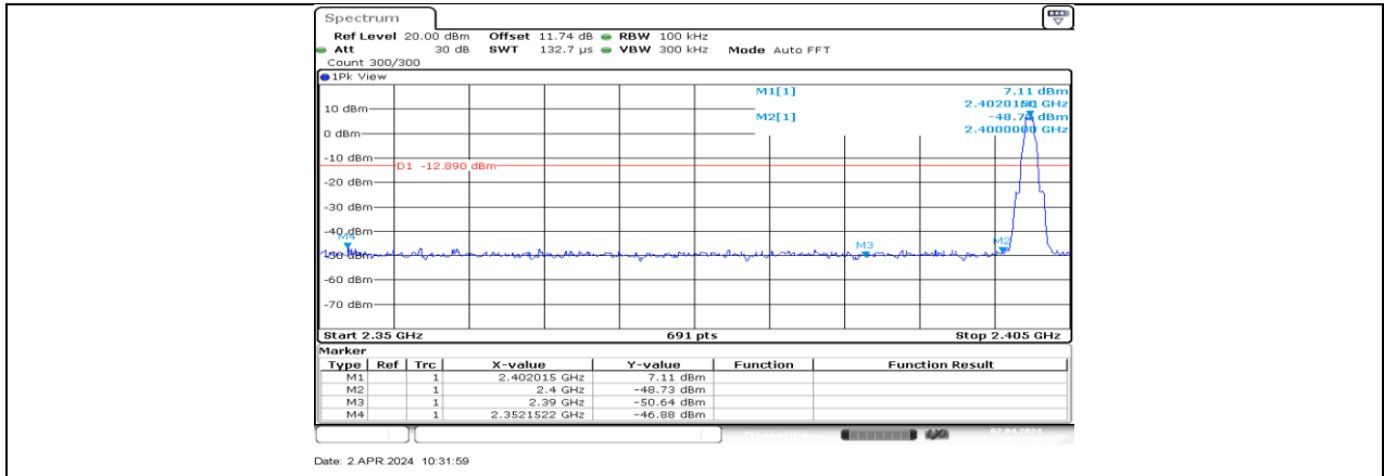
BLE_1M_Ant1_Low_2402
