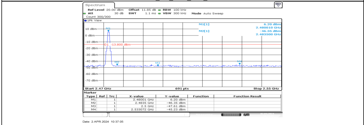
BLE_1M_Ant1_High_2480
