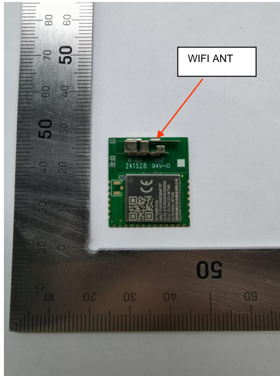
View of EUT-1
