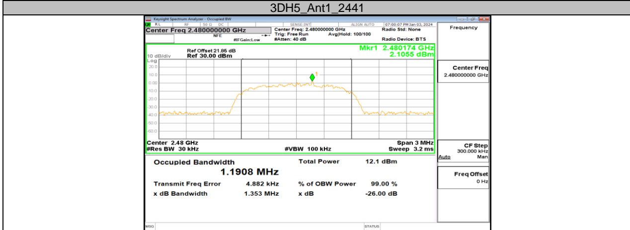
3DH5_Ant1_2480
