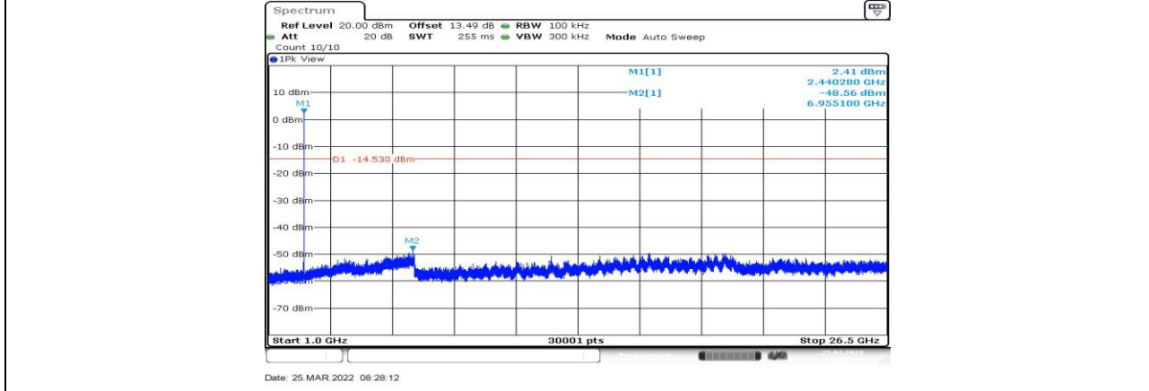
BLE_2M_Ant1_2440_1000~26500
