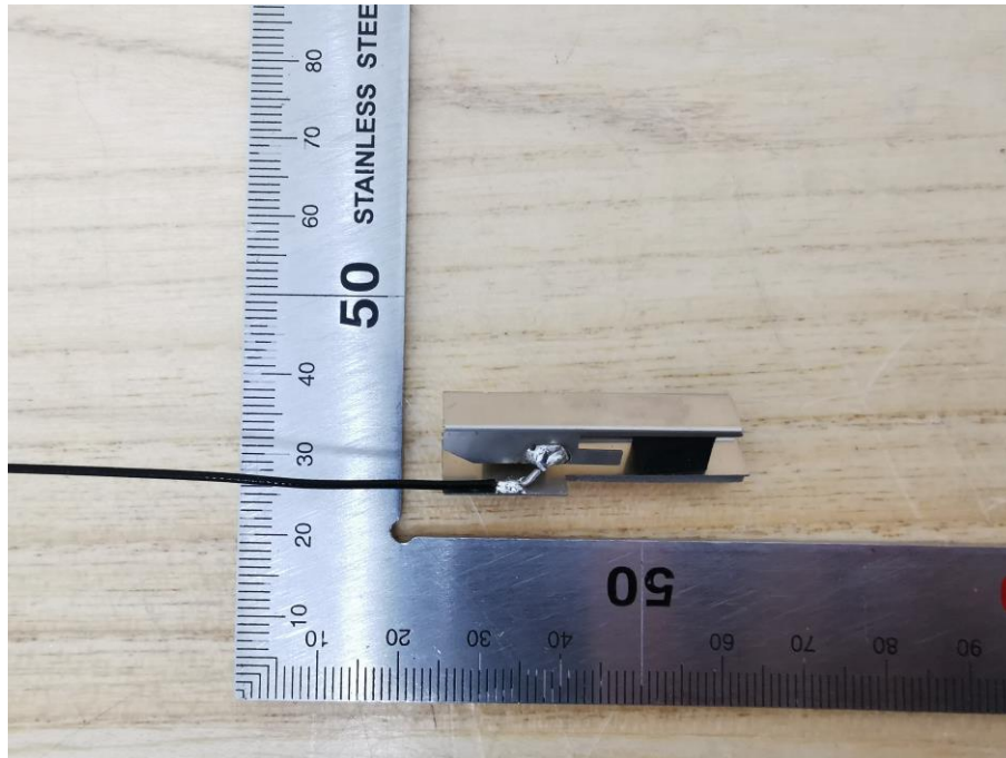
View of EUT-12 ANT WCT5J
