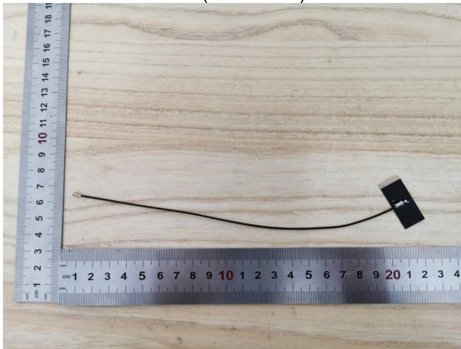
View of EUT-4 ANT(WCT5H-20)
