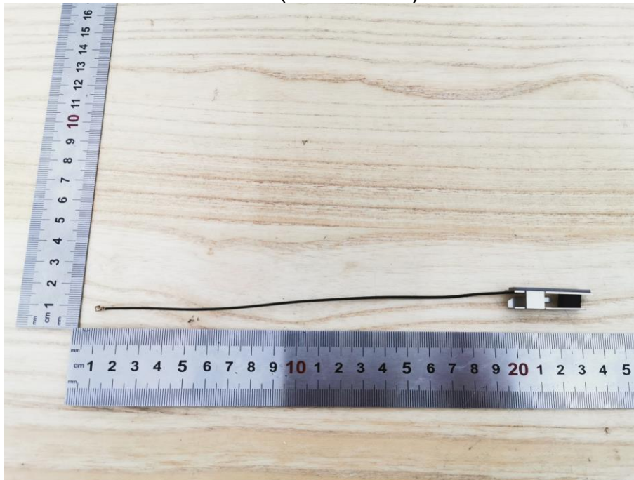
View of EUT-10 ANT(WCT5J-40)
