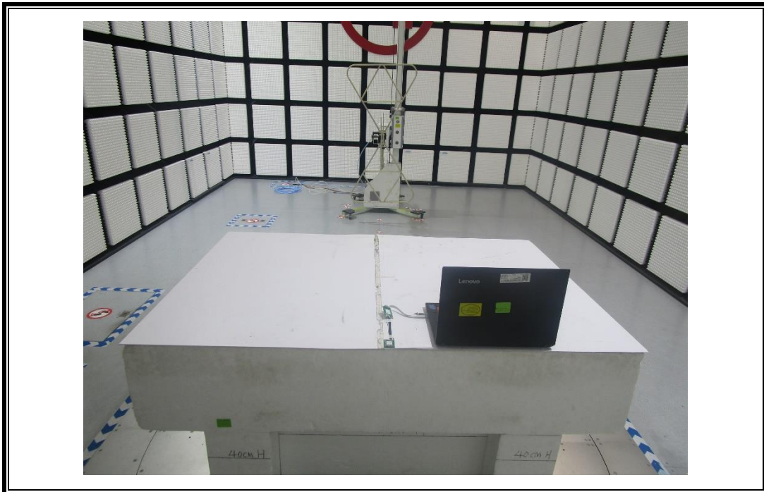
RADIATED RF MEASUREMENT SETUP (Below 1 GHz and Above 30 MHz)
