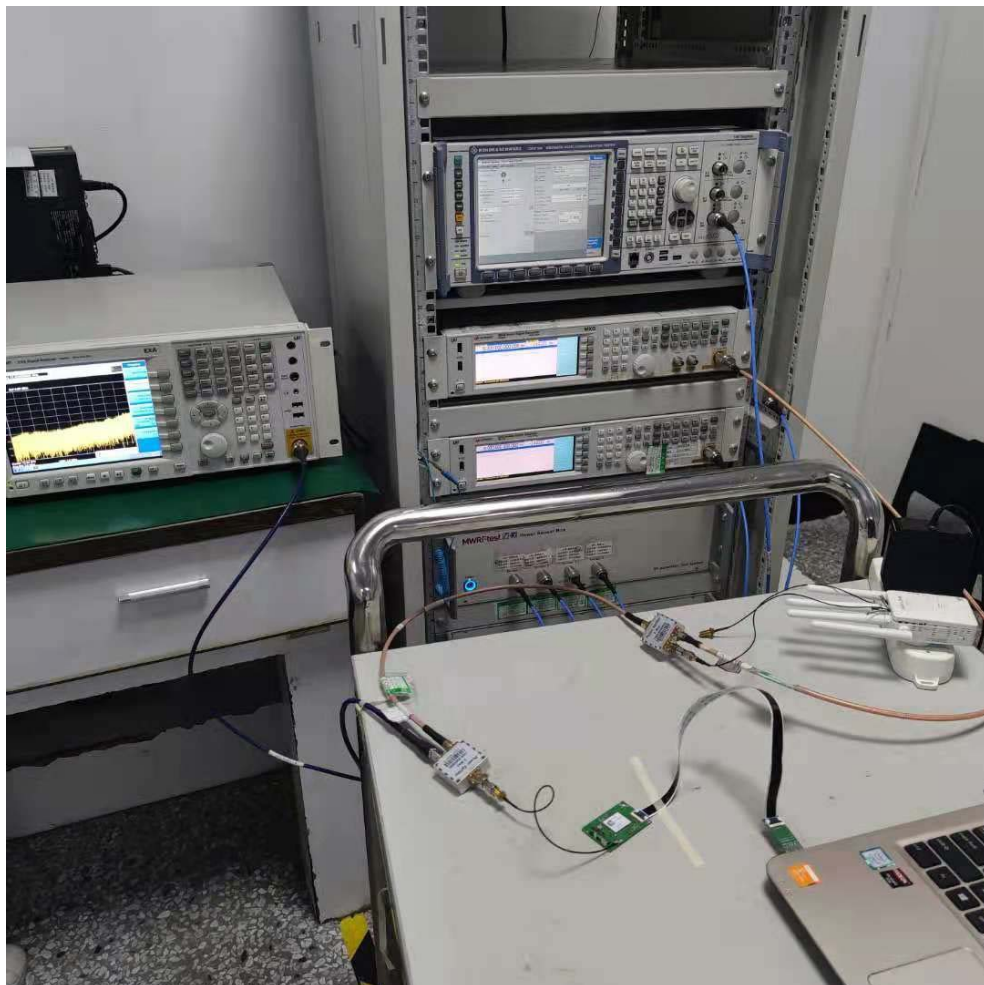
DFS Test Photo
