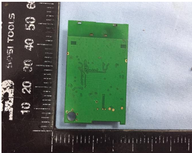
EUT View 2
