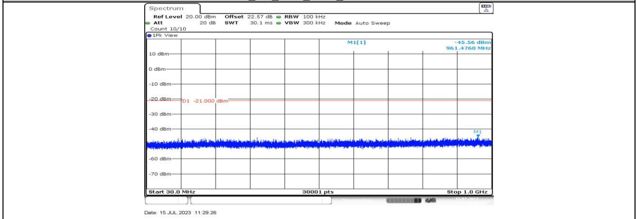
BLE_2M_Ant1_2440_30~1000
