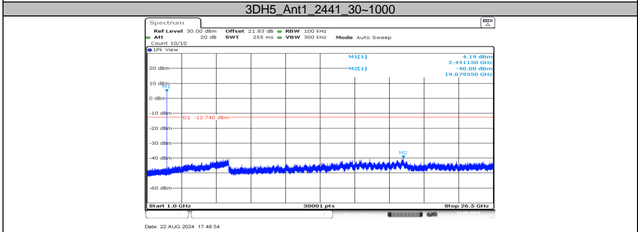
3DH5_Ant1_2441_1000~26500
