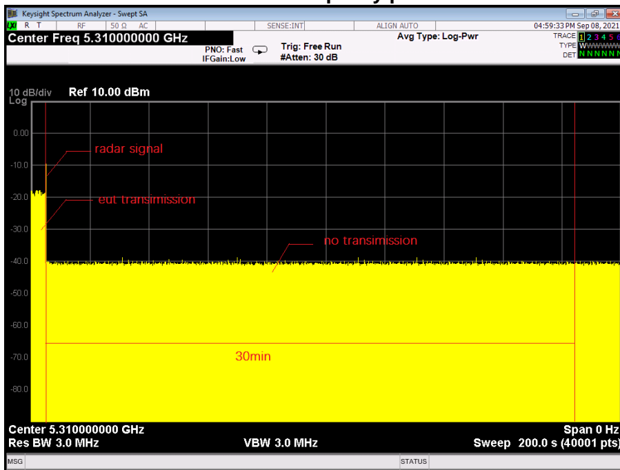
TX AC (VHT40) Mode 5310 Non-Occupancy period
