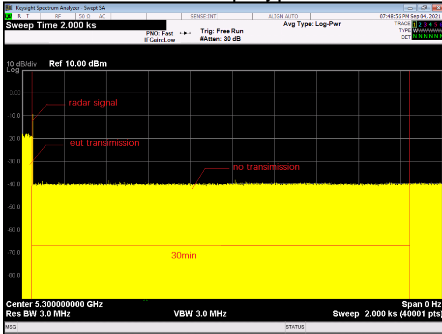
TX AC(VHT20) Mode 5300 Non-Occupancy period
