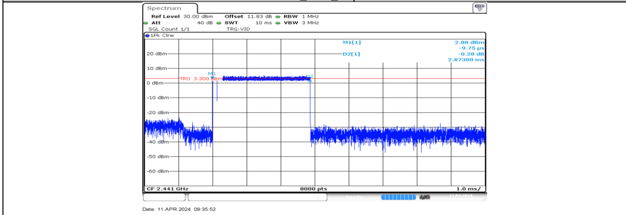
3DH5_Ant3_Hop
