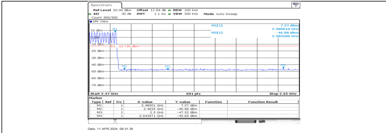
DH5_Ant3_High_Hop_2480
