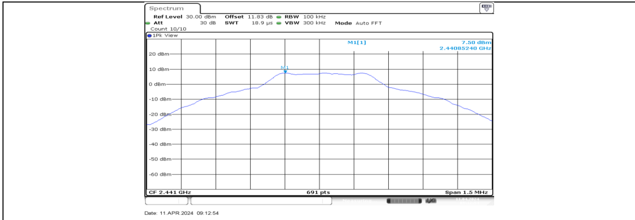
DH5_Ant3_2441_0~Reference
