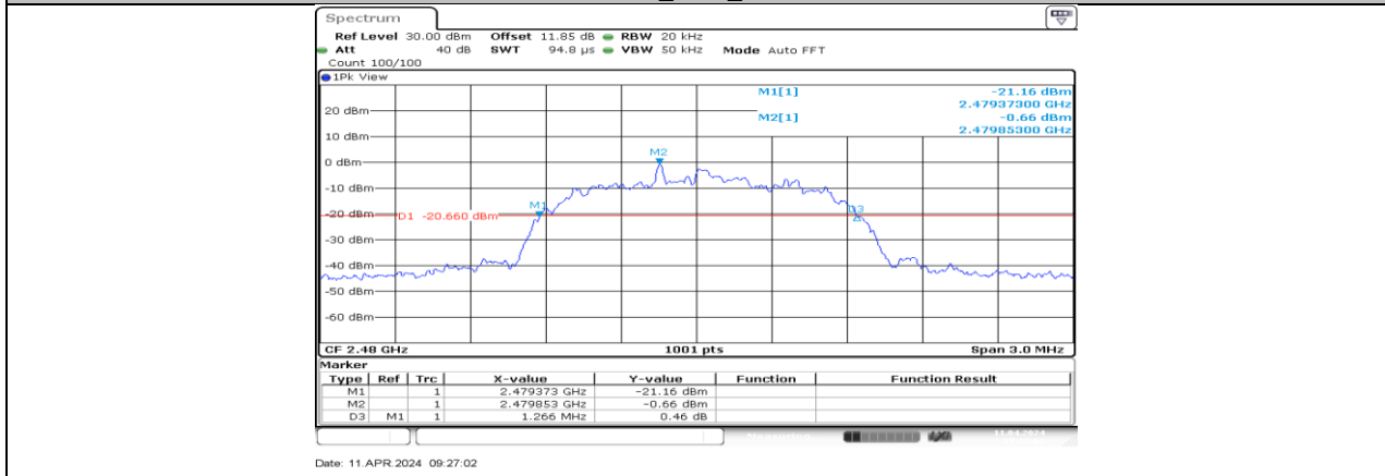
3DH5_Ant3_2480
