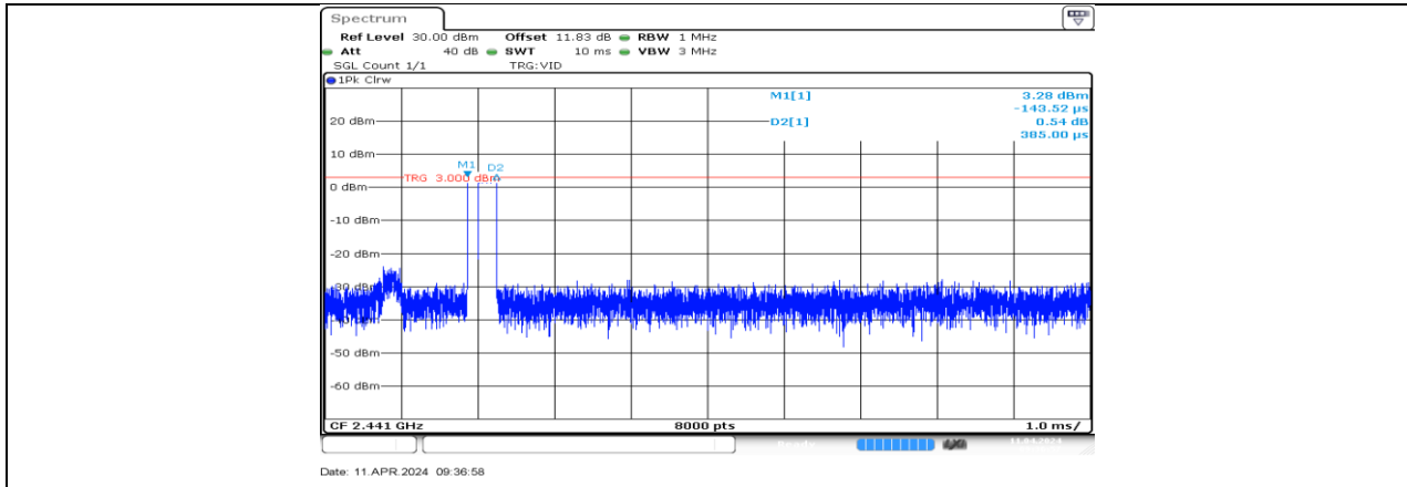
3DH1_Ant3_Hop
