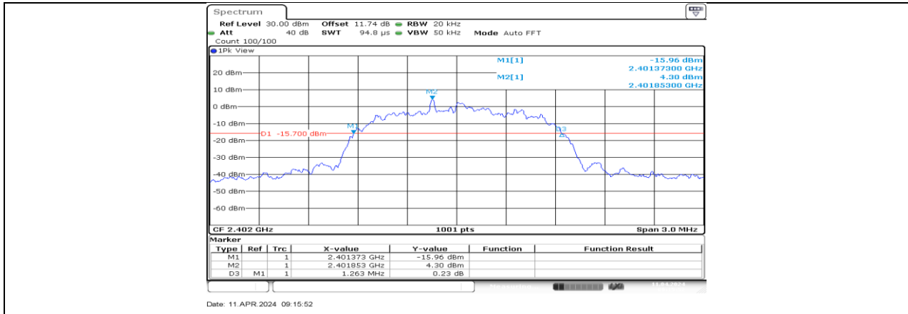
3DH5_Ant3_2402
