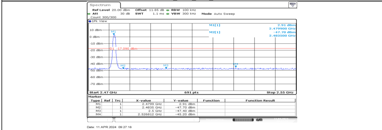
3DH5_Ant3_High_2480
