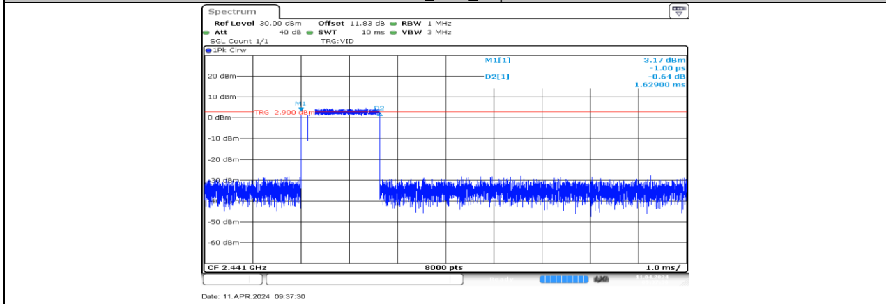
3DH3_Ant3_Hop
