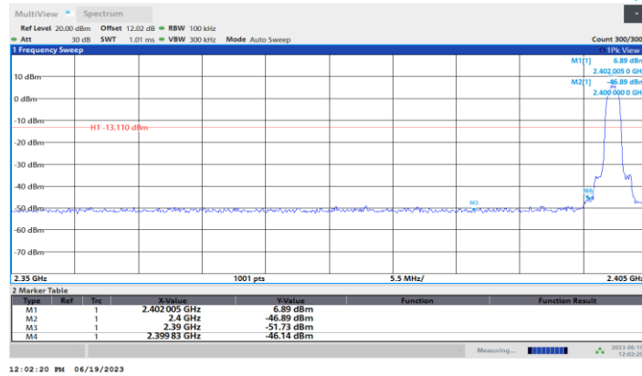
3DH5_Ant1_Low_2402
