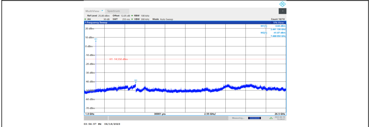
DH5_Ant1_2441_1000~26500
