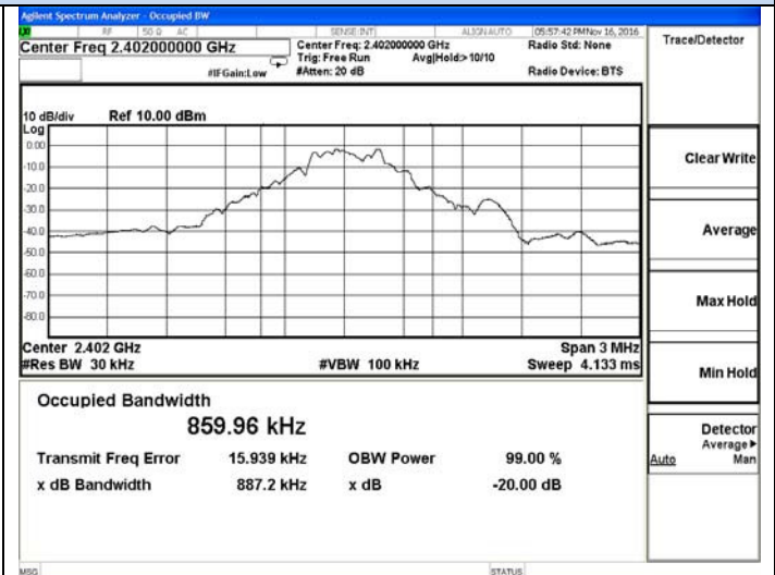
20dB Bandwidth GFSK-Low channel
