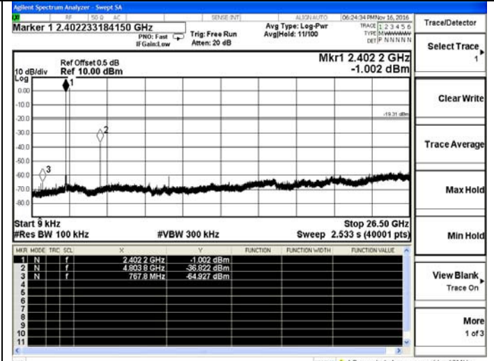
GFSK -Low channel
