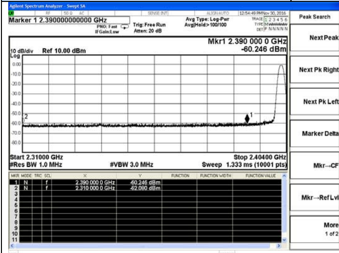
GFSK-Low channel(Peak)
