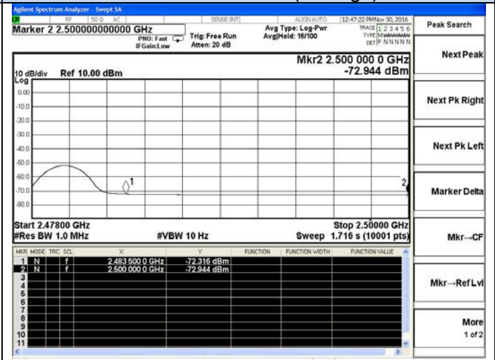
GFSK -High channel(Average)
