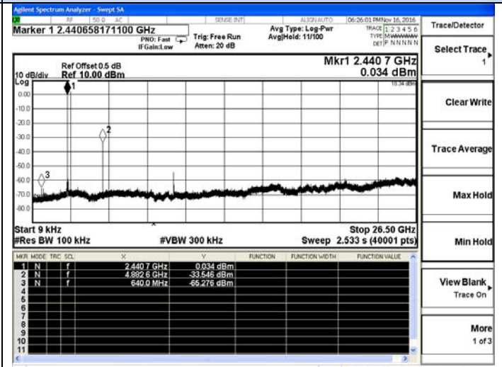
GFSK -Middle channel
