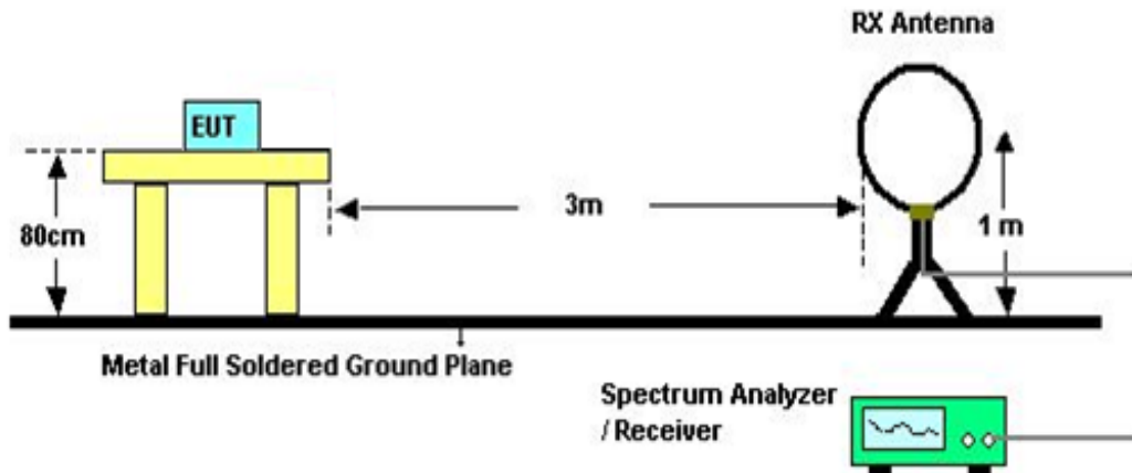
(C) Radiated emissions below 30 MHz
