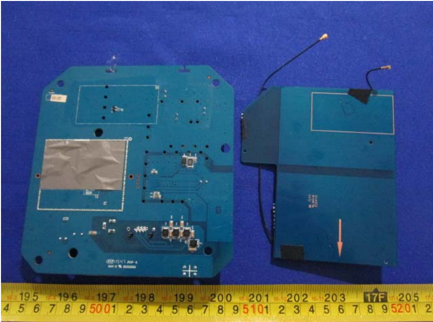
EUT –PCB Board Uncover View
