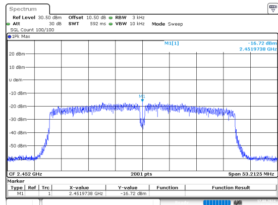
n40_2452MHz_Chain 1
