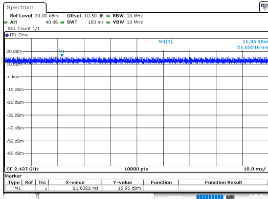
n20_2437MHz
