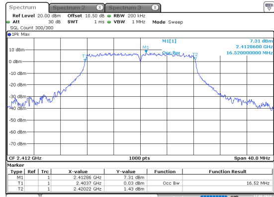
g_2412MHz
