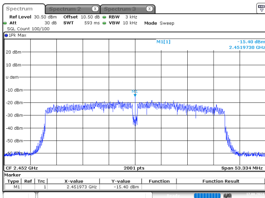
n40_2452MHz_Chain 0
