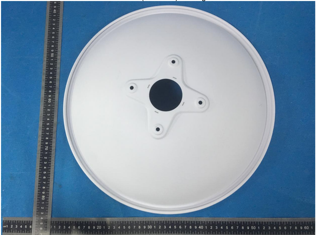
Photo4 External (Screw on) Cassegrain Antenna
