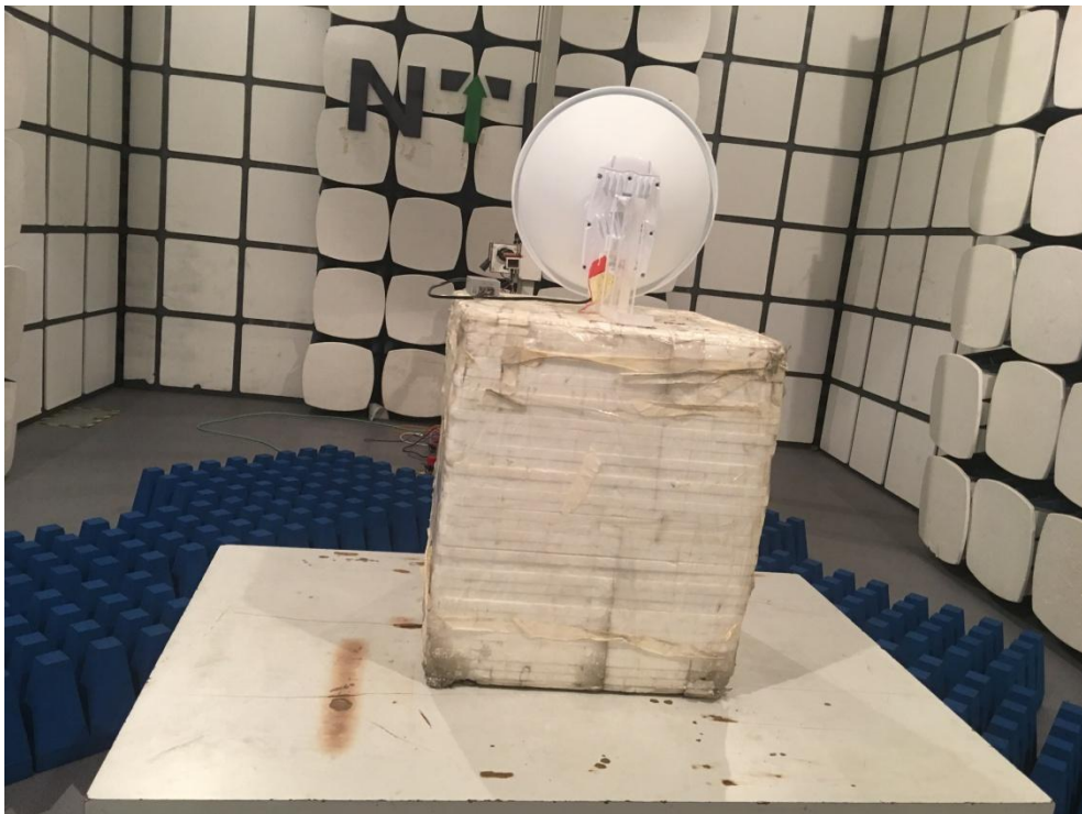
(18GHz~40GHz) 25dBi Antenna
