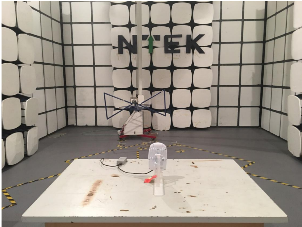
Radiated Measurement Photos (30MHz~1GHz ) 8dBi Antenna
