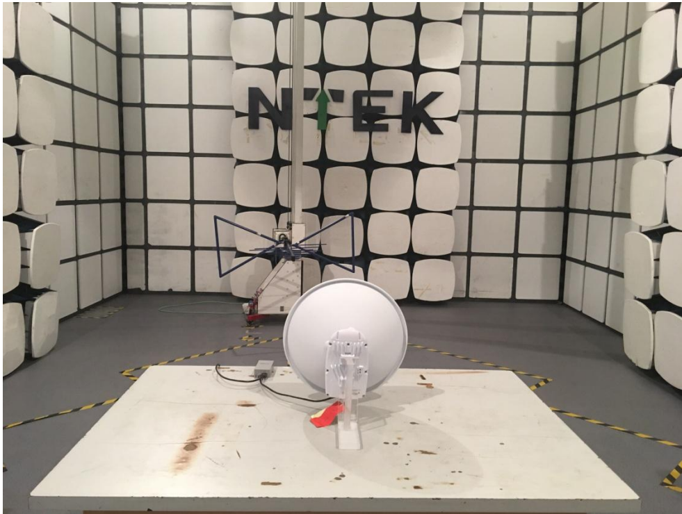
Radiated Measurement Photos (30MHz~1GHz) 25dBi Antenna
