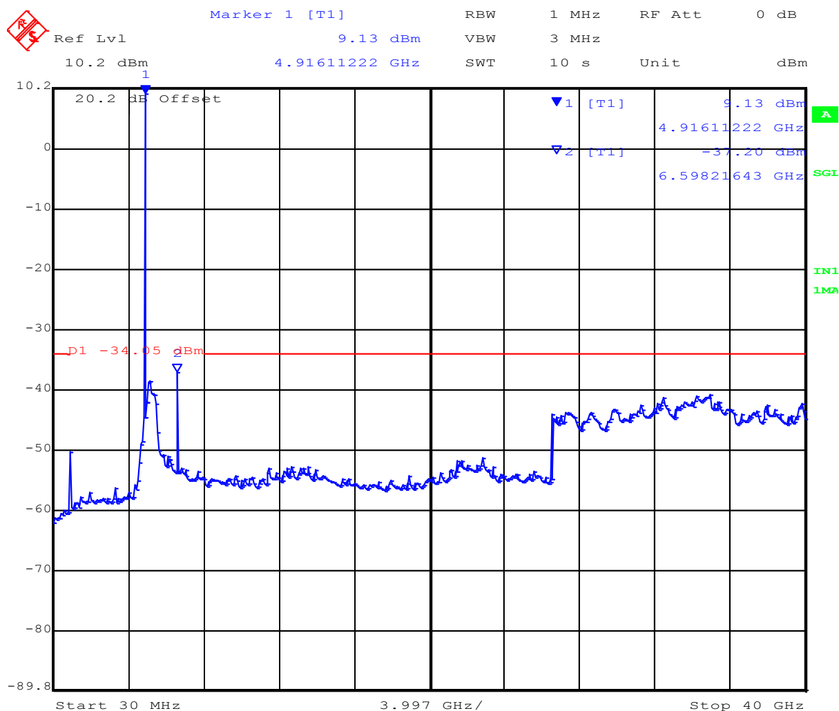
Port A Conducted Emissions Channel Freq 4950 MHz
