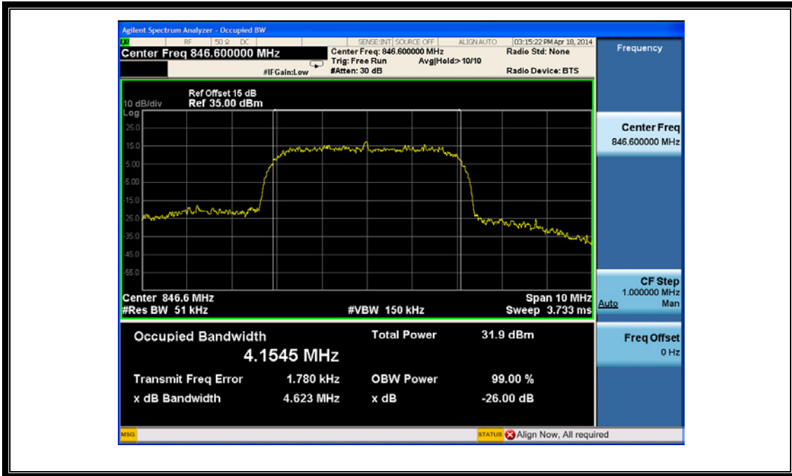
(Plot C: WCDMA 850MHz Channel = 4233)
