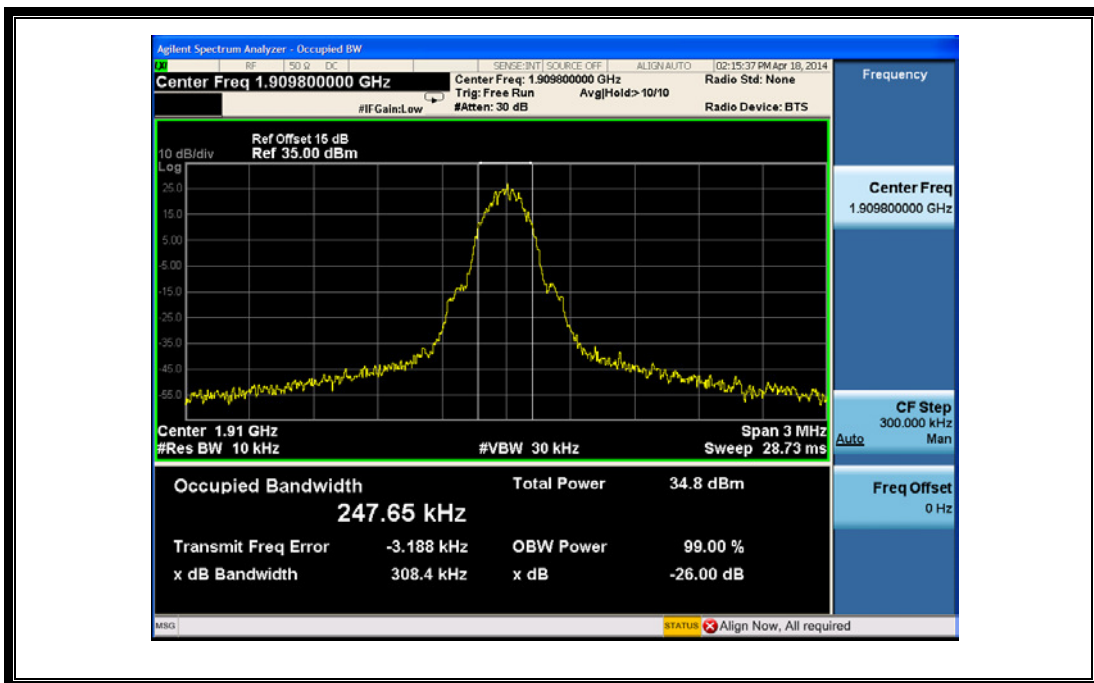
(Plot L1: GSM 1900MHz Channel = 810)
