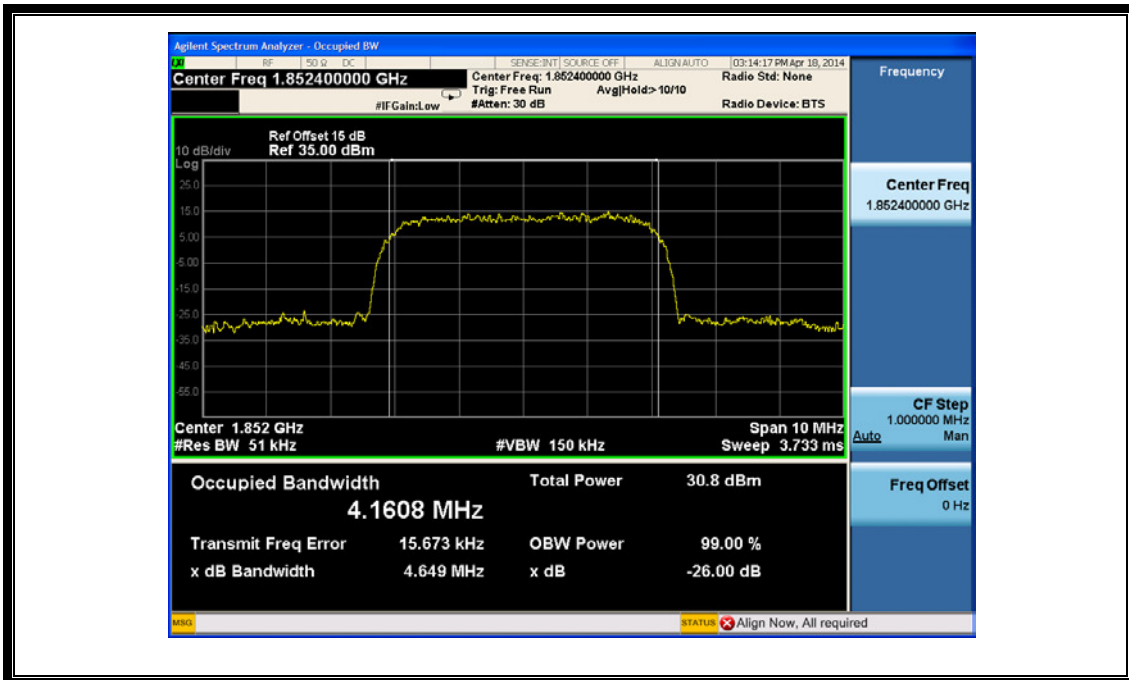
(Plot D: WCDMA 1900MHz Channel = 9262)
