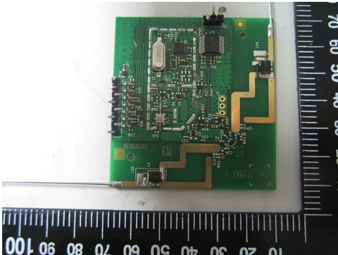
6. GSM antenna view
