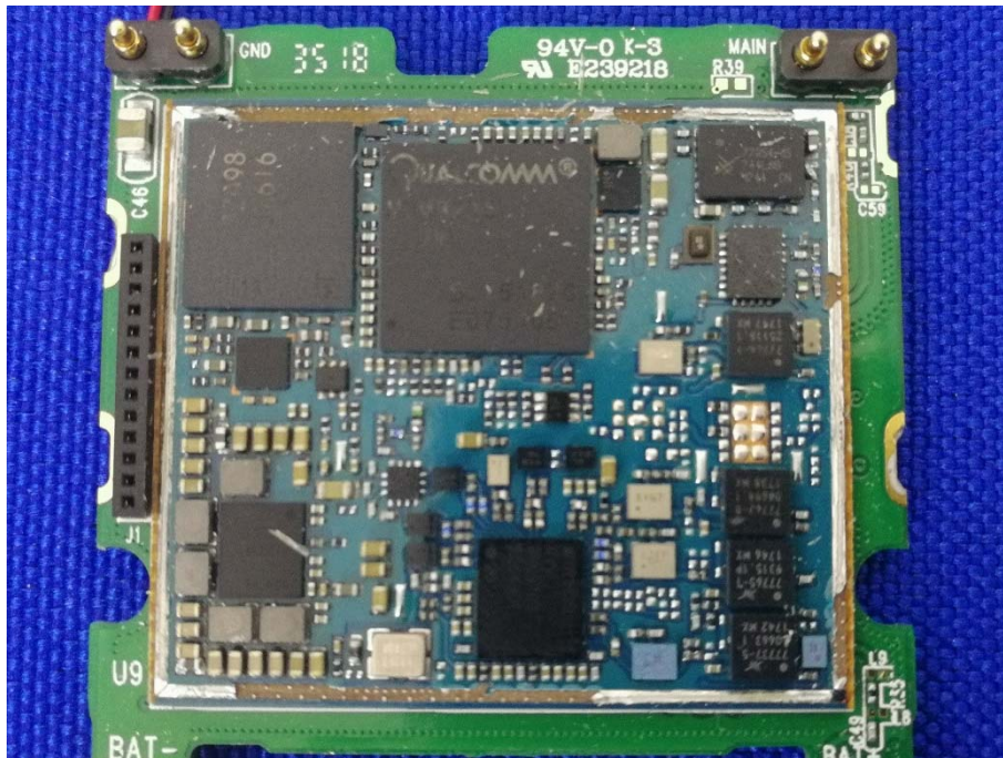
MAIN BOARD REAR VIEW (CLOSE-UP)
