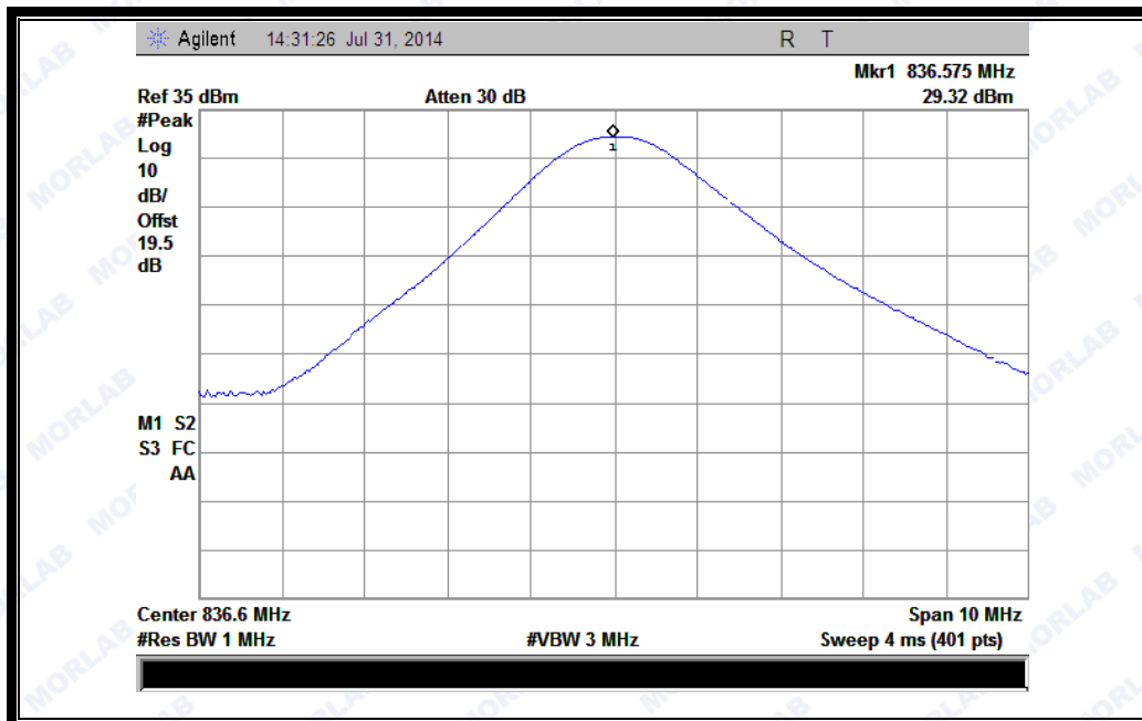
(Plot C 2: GPRS 850MHz Channel = 190)
