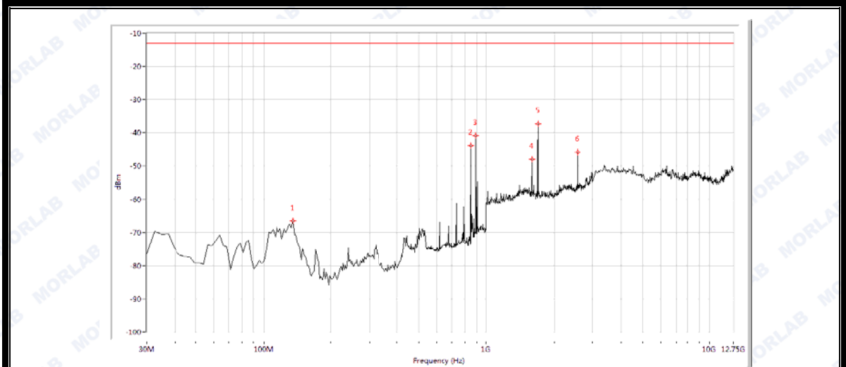
(Plot C.4: EGPRS 850MHz Channel = 190, Test Antenna Vertical)
