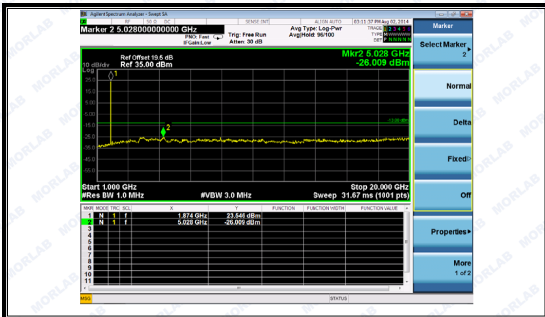
(Plot F2.1: WCDMA1900MHz Channel = 9400, 1GHz to 20GHz)
