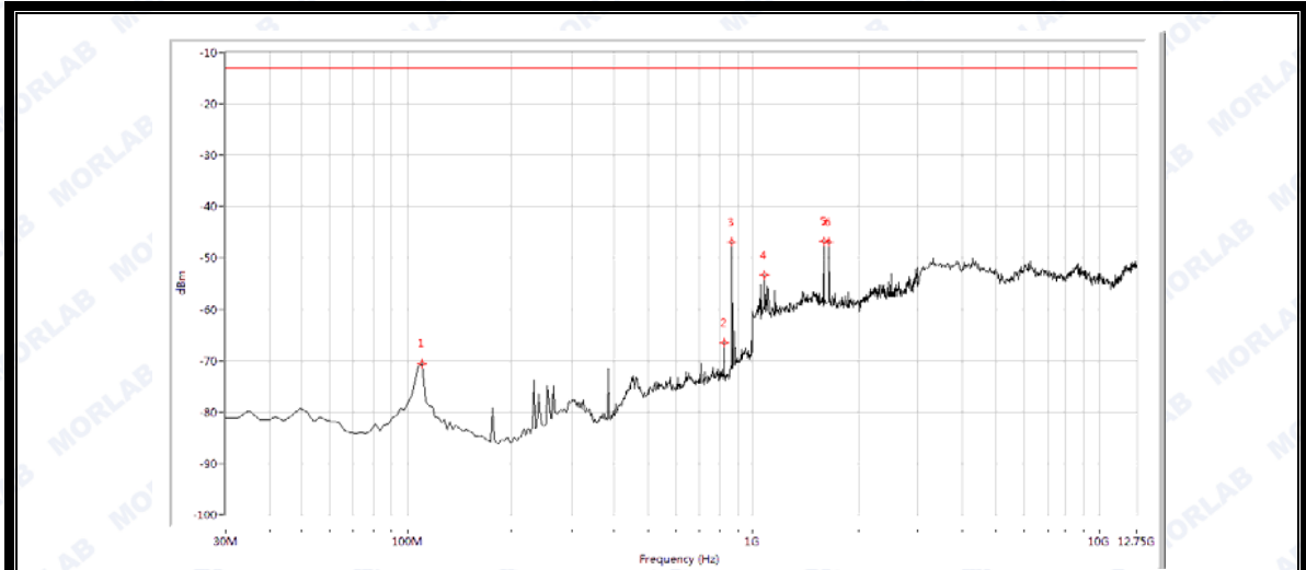
(Plot C.1: EGPRS 850MHz Channel = 128, Test Antenna Horizontal)
