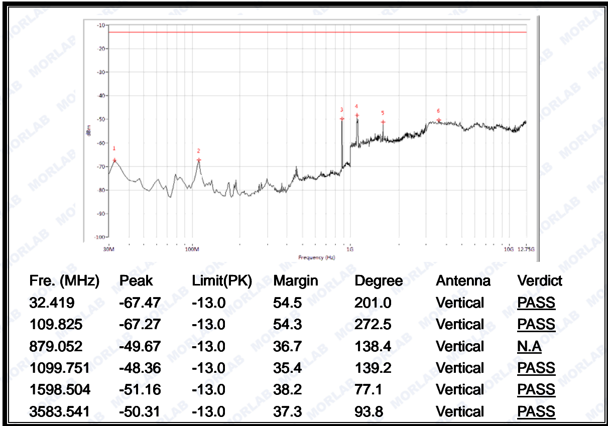
(Plot E.4: WCDMA 850MHz Channel = 4175, Test Antenna Vertical)
