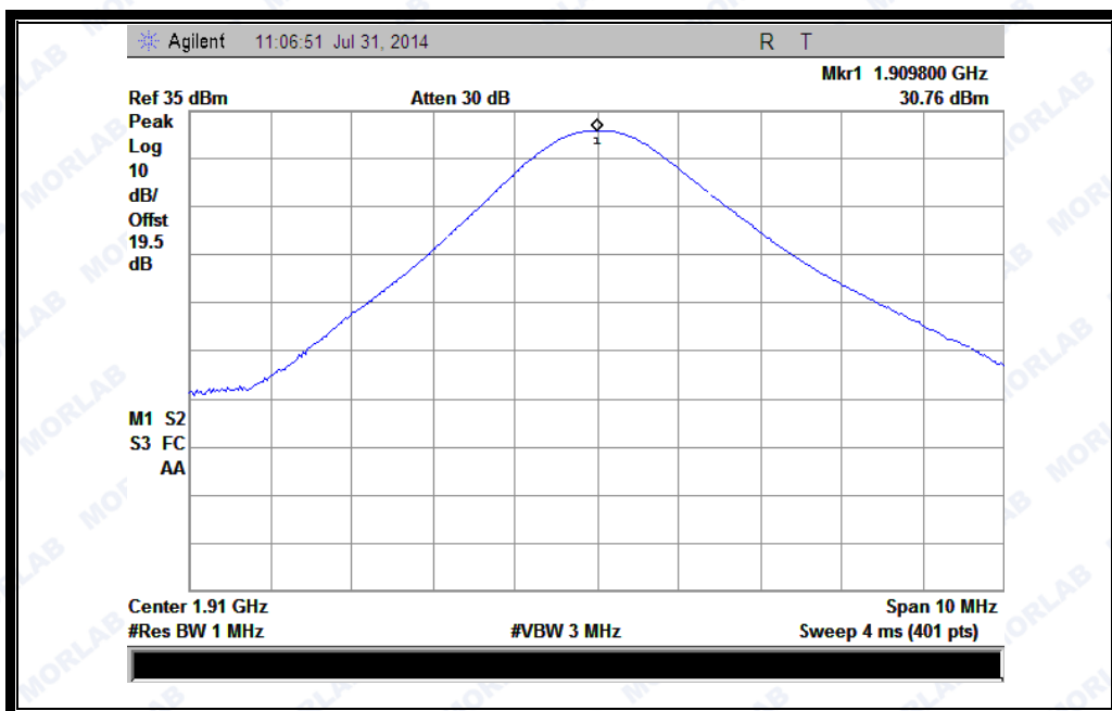
(Plot B3: GSM 1900MHz Channel = 810)
