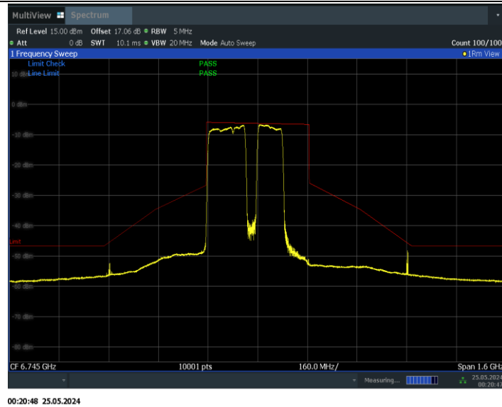
11BE320MIMO_Ant1_6745_2*996+484_Non-OFDMA_5
