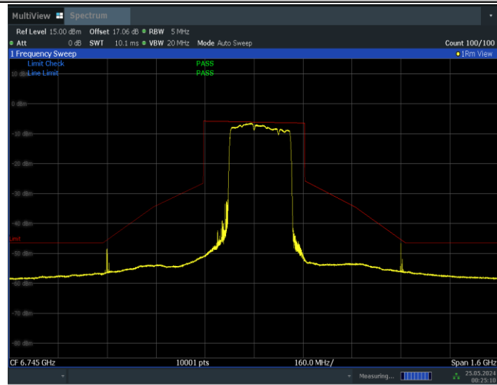
11BE320MIMO_Ant1_6745_2*996+484_Non-OFDMA_12
