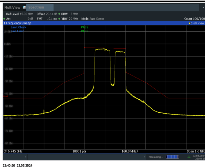
11BE320MIMO_Ant0_6745_2*996+484_Non-OFDMA_10
