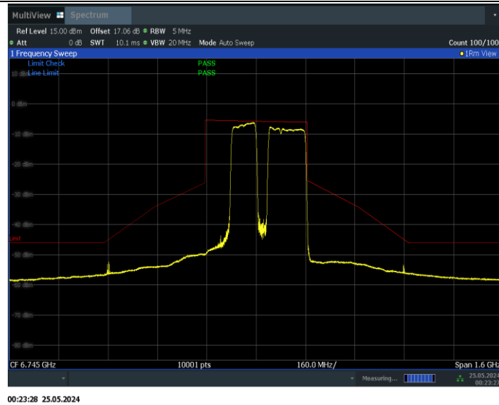
11BE320MIMO_Ant1_6745_2*996+484_Non-OFDMA_10
