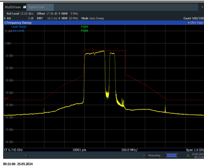
11BE320MIMO_Ant1_6745_2*996+484_Non-OFDMA_6
