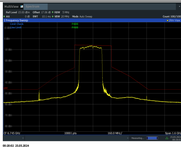
11BE320MIMO_Ant1_6745_2*996+484_Non-OFDMA_1
